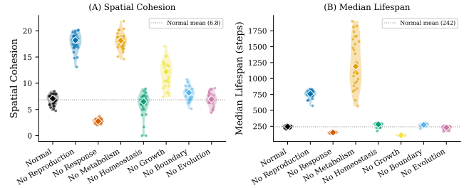
Figure 5: Criterion-orthogonal outcome measures ( n=30 per condition). Left: spatial cohesion (mean pairwise agent distance); lower values indicate tighter spatial structure. Right: median organism lifespan per seed. Diamonds mark medians; dotted line shows normal baseline. Response ablation significantly increases cohesion (immobile organisms cluster) while decreasing lifespan.
