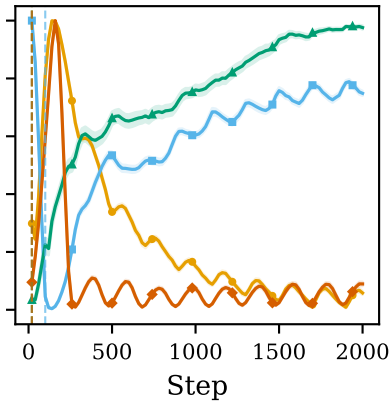
Response Ablation
