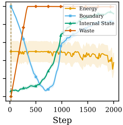
Reproduction Ablation
