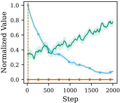
Metabolism Ablation
