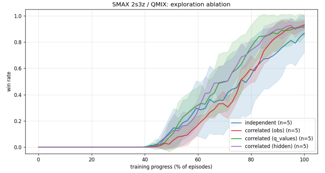
Figure 3: SMAX 2s3z (QMIX). Correlated variants reach a higher final win rate than independent (0.91 vs. 0.81) and get there sooner.
