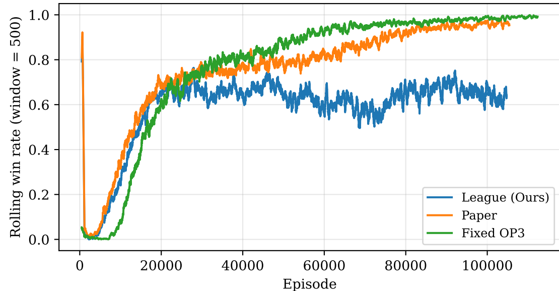
4v4 training: win rate over time
