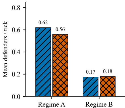
(a) Defender allocation
