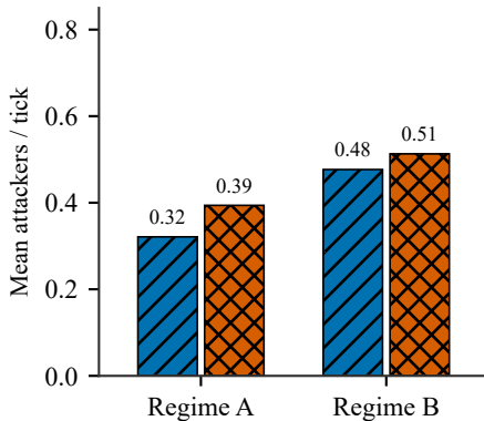
(b) Attacker allocation
