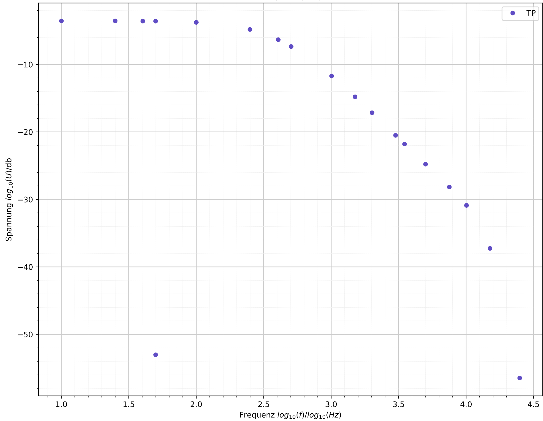
Frequenzgang
