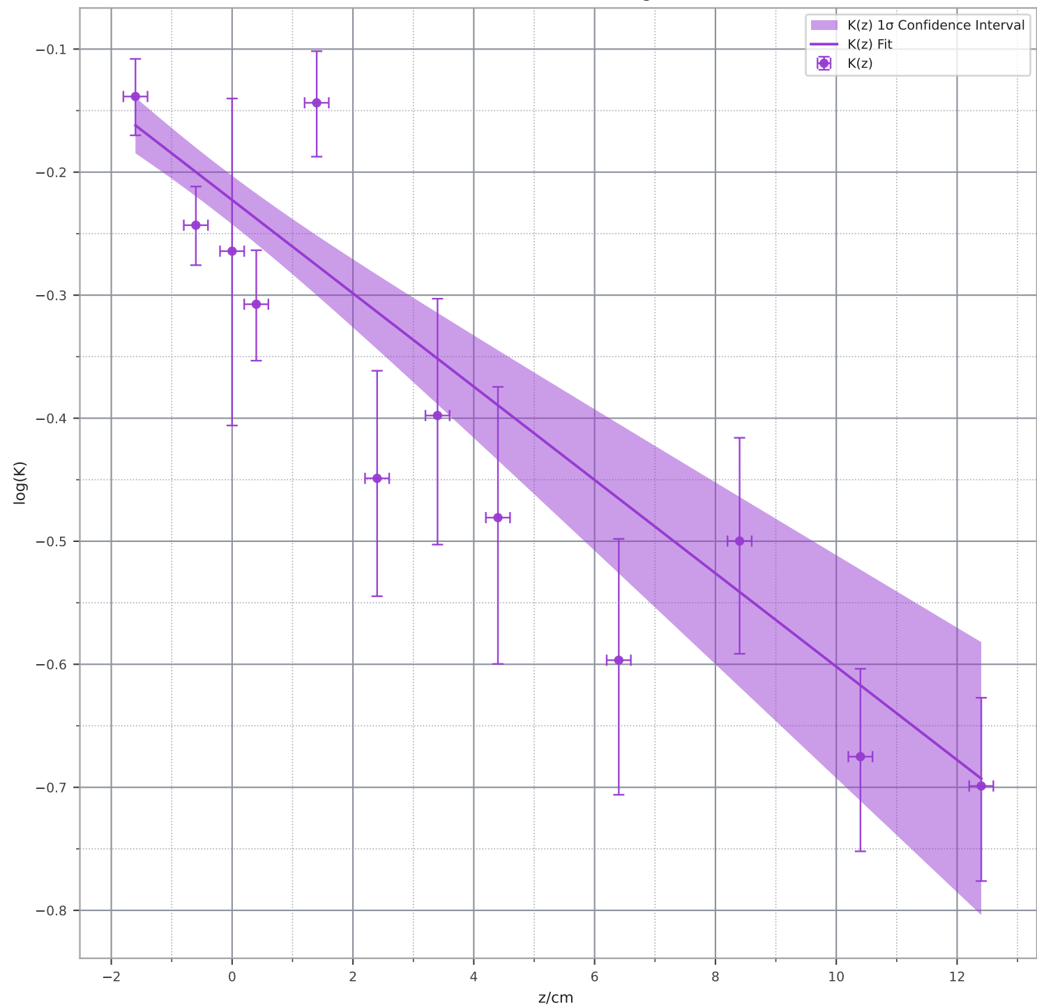
Michelson Interferometer - log(Kontrast)
