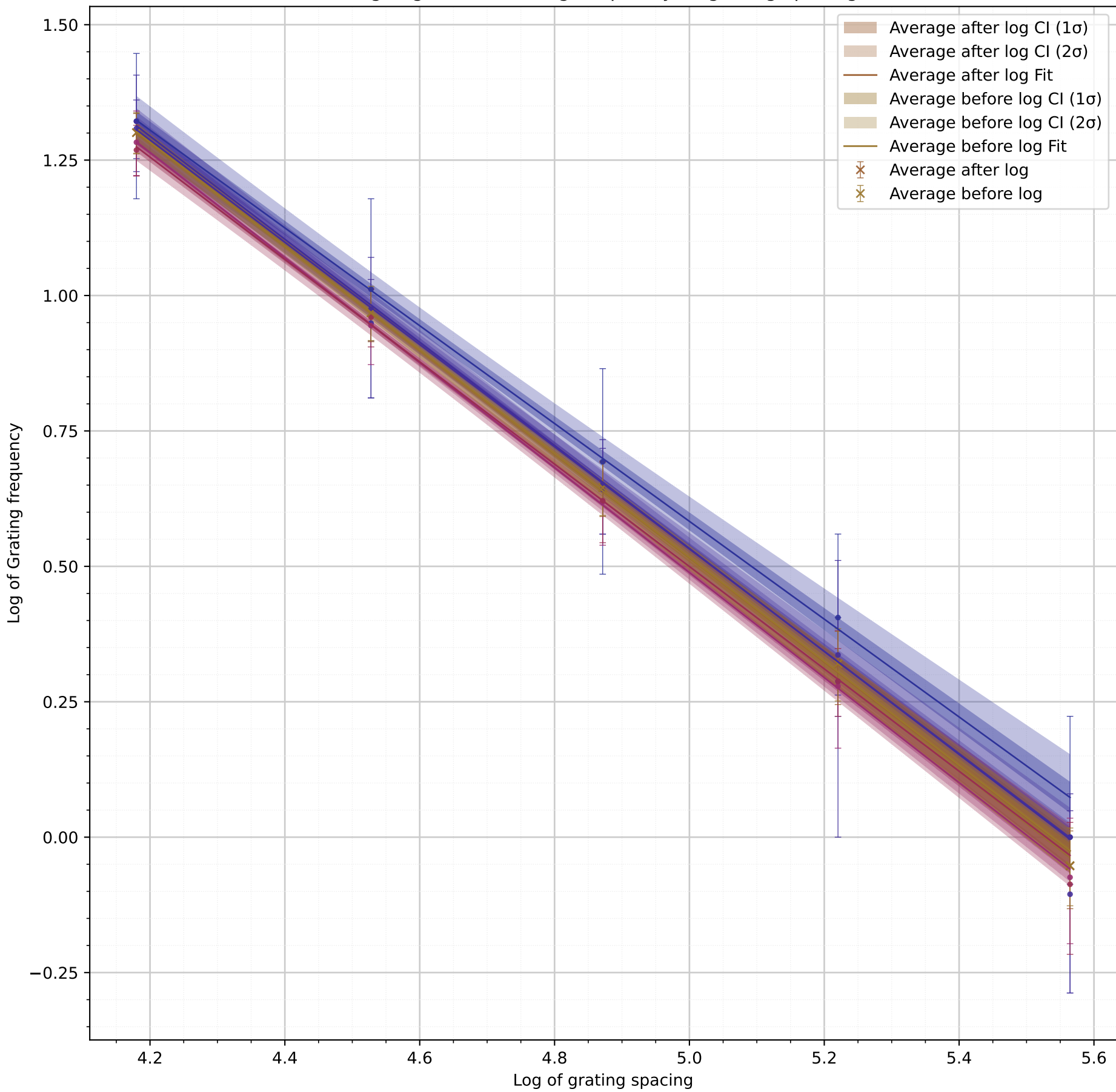
Log-Log Plot of Grating frequency vs grating spacing
