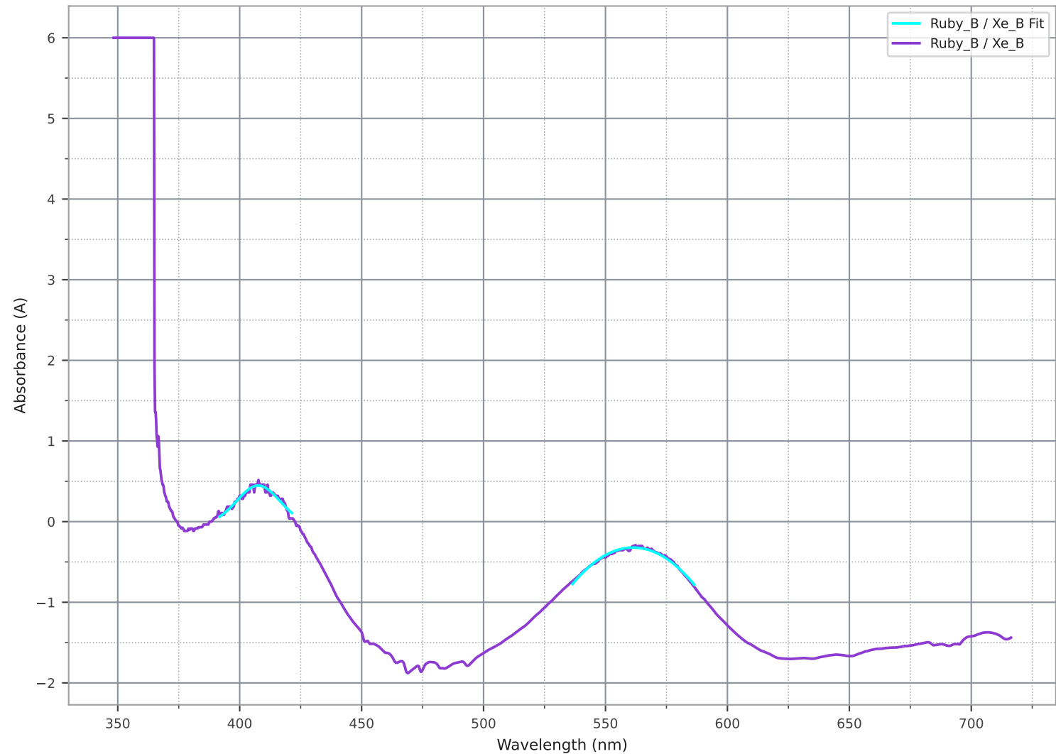
Ruby Data: Absorbance Ruby / Xe Spectra
