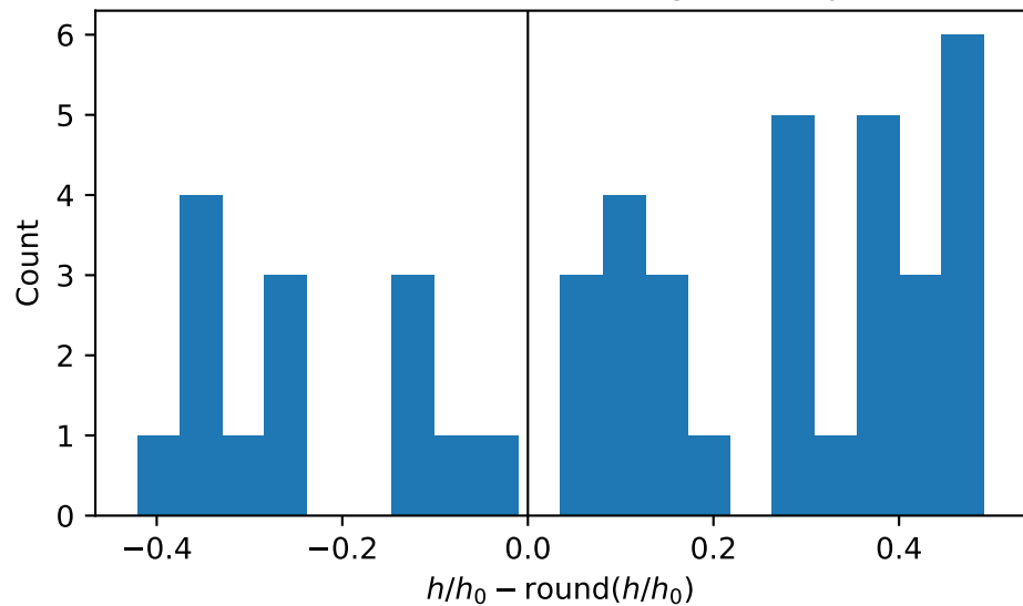
Distance to nearest integer multiple
