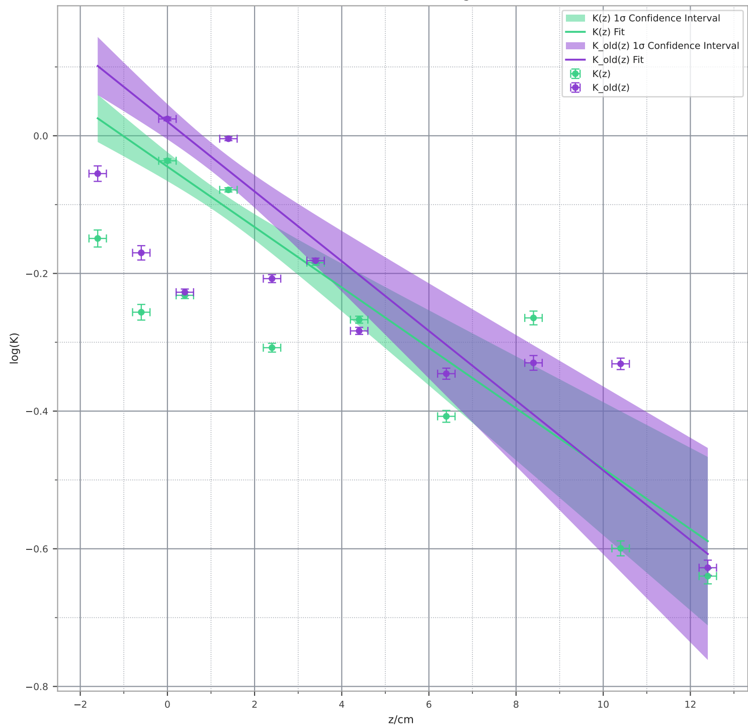
Michelson Interferometer - \log(\text{Kontrast})
