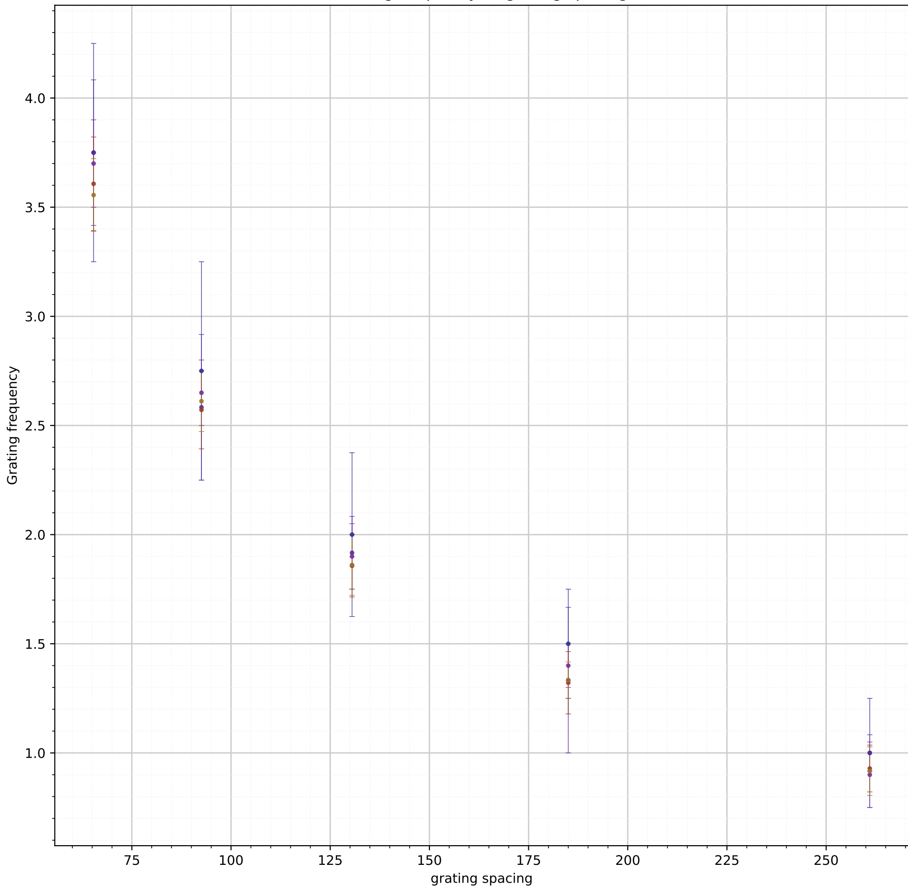
Grating frequency vs grating spacing
