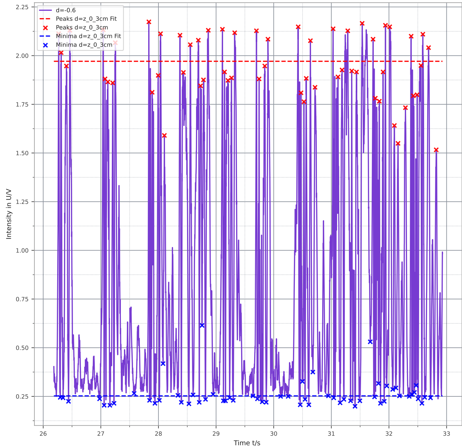
Michelson Interferometer
