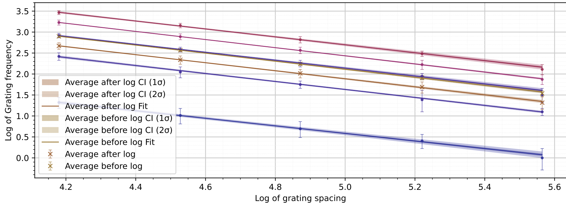
Log-Log Plot of Grating frequency vs grating spacing
