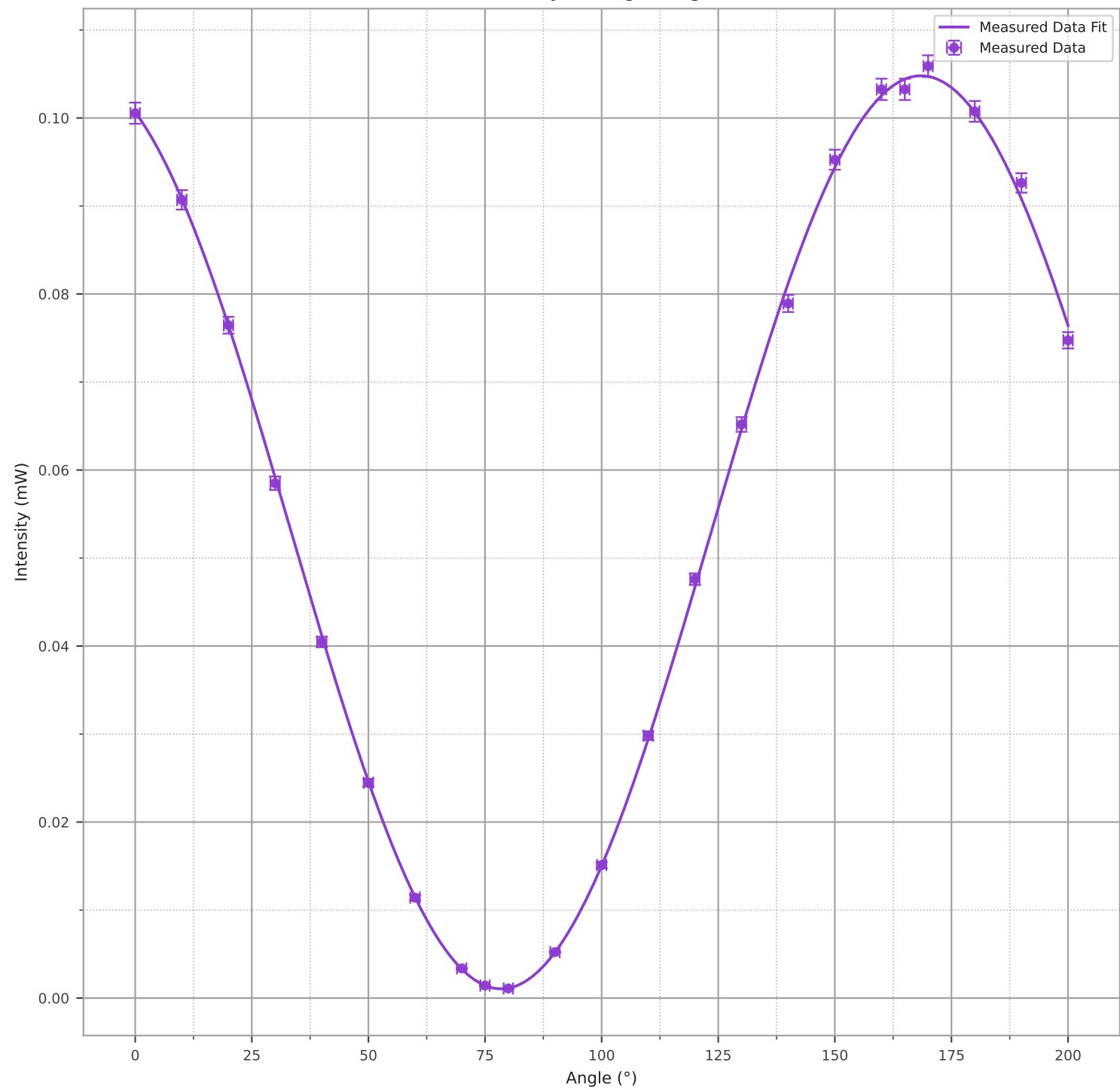
Laser Intensity vs Angle (High Power)
