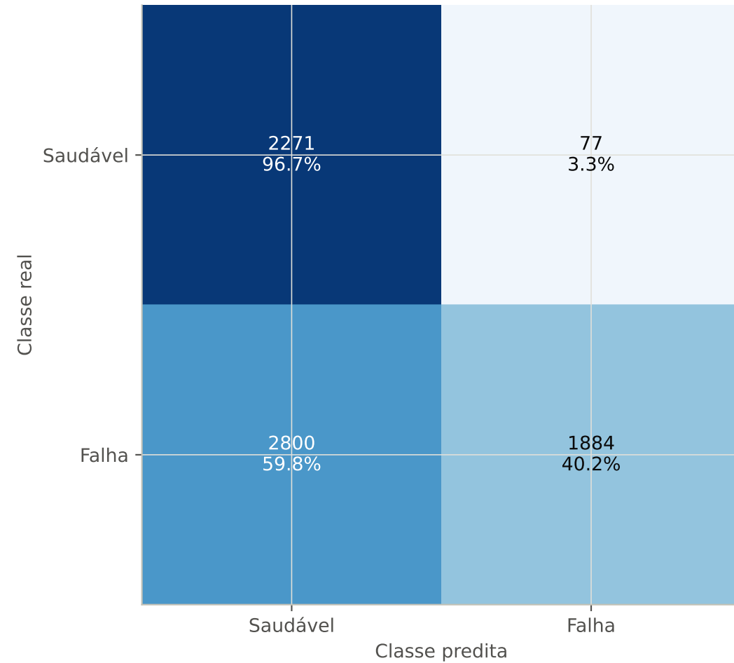
AE-LSTM
