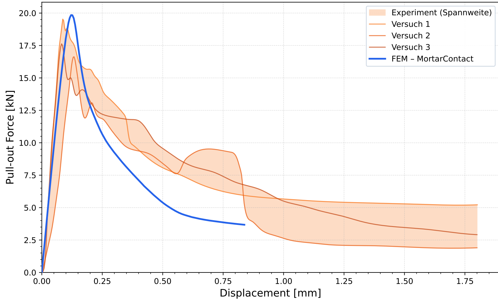
VA1 - Pull-Out Test: EBT 6cm MortarContact3D vs. Experiment
