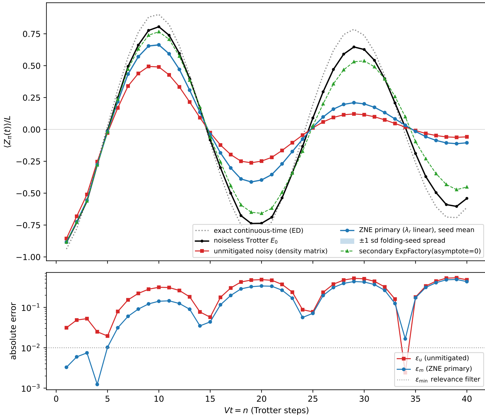
MFIM scar dynamics under two-tier depolarizing noise, L = 6 , V = 1 , \Omega = 0.24 , \Delta t = 1 (design §15)
