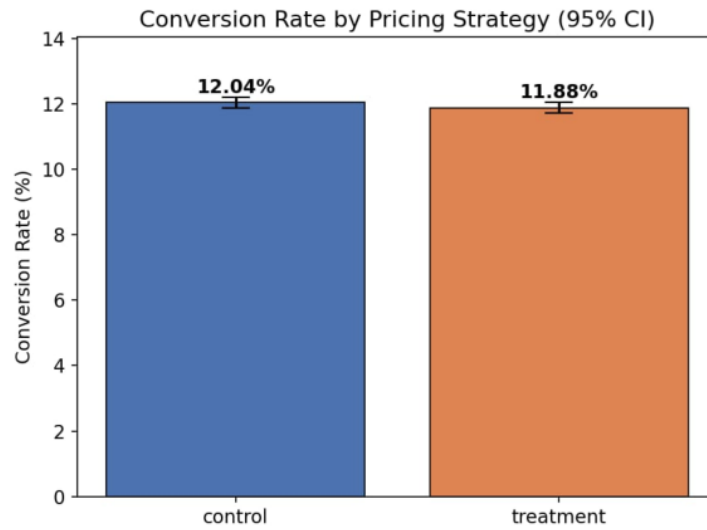
Figure 2: Conversion rate by pricing strategy, with 95% confidence intervals. The intervals overlap substantially, hinting the difference may not be statistically meaningful.
