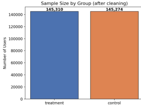
Figure 1: Sample size per group after cleaning. The near-identical group sizes confirm the random assignment worked as intended.
