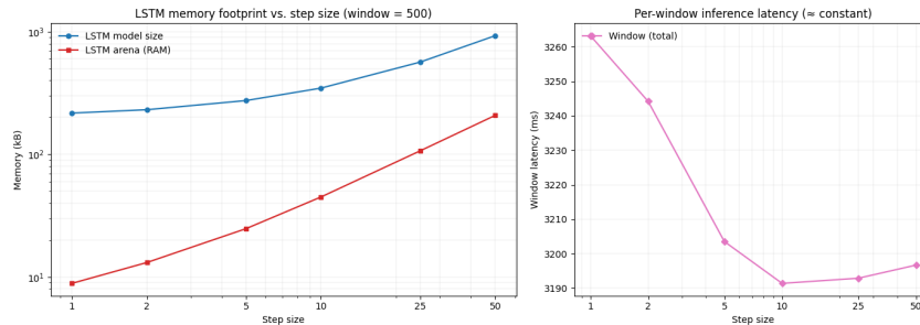
Figure 6.3: LSTM memory footprint and per-window inference latency as a function of step size, at a fixed window length of 500 samples. Memory (left, log scale) grows steeply with step size for both the model and the activation arena, whereas the per-window latency (right) remains essentially constant, varying by under 3% across the full range. Note that the latency axis is zoomed; the apparent dip corresponds to an absolute change of only a few tens of microseconds.
