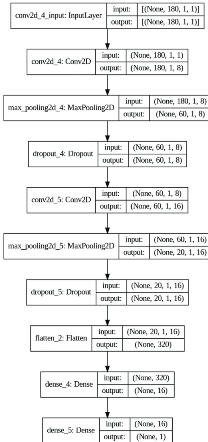
Figure 2.2: Convolutional–fully-connected architecture employed by Kim et al. [25].
