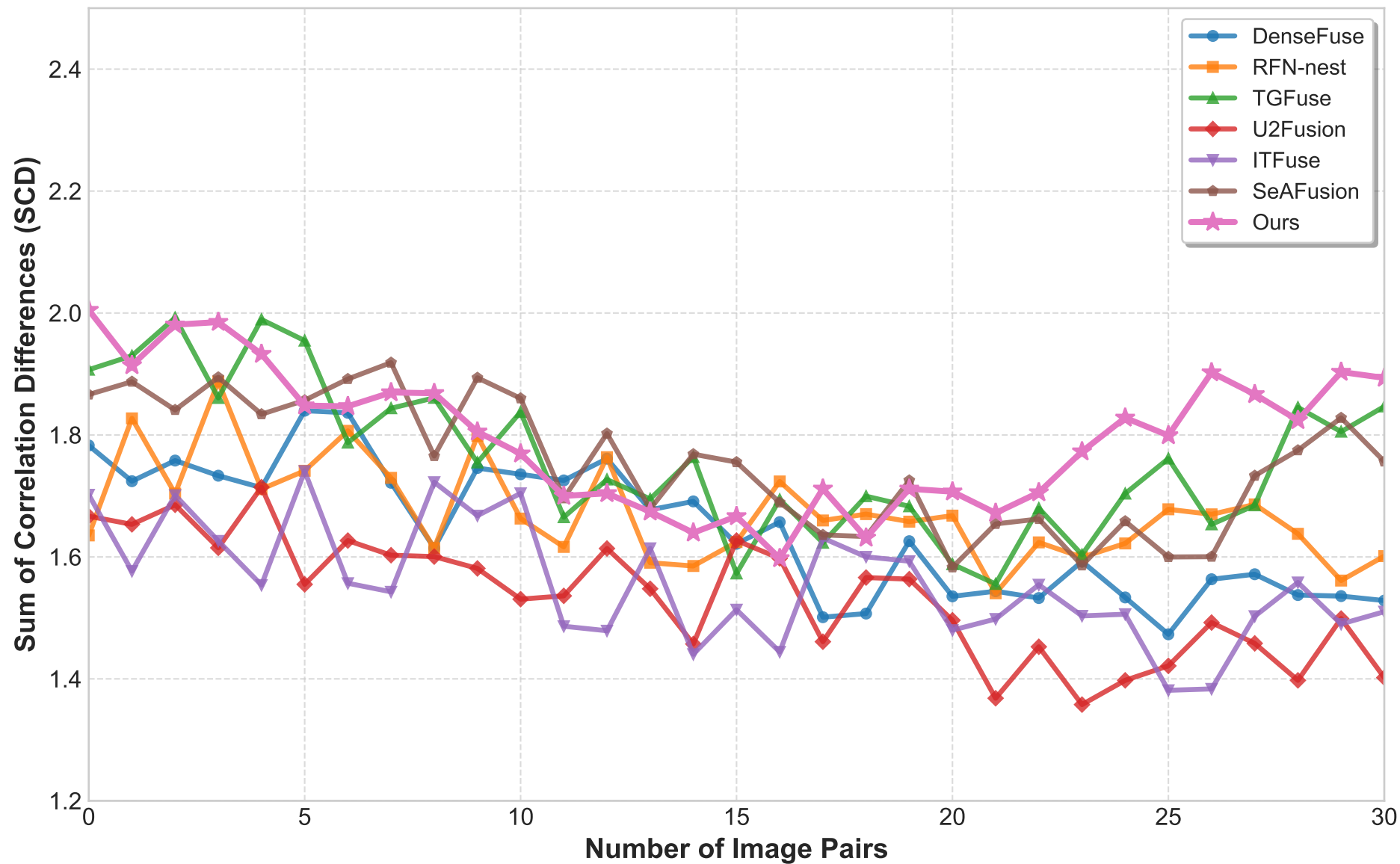
Sum of Correlation Differences (SCD) Comparison (Higher is Better)
