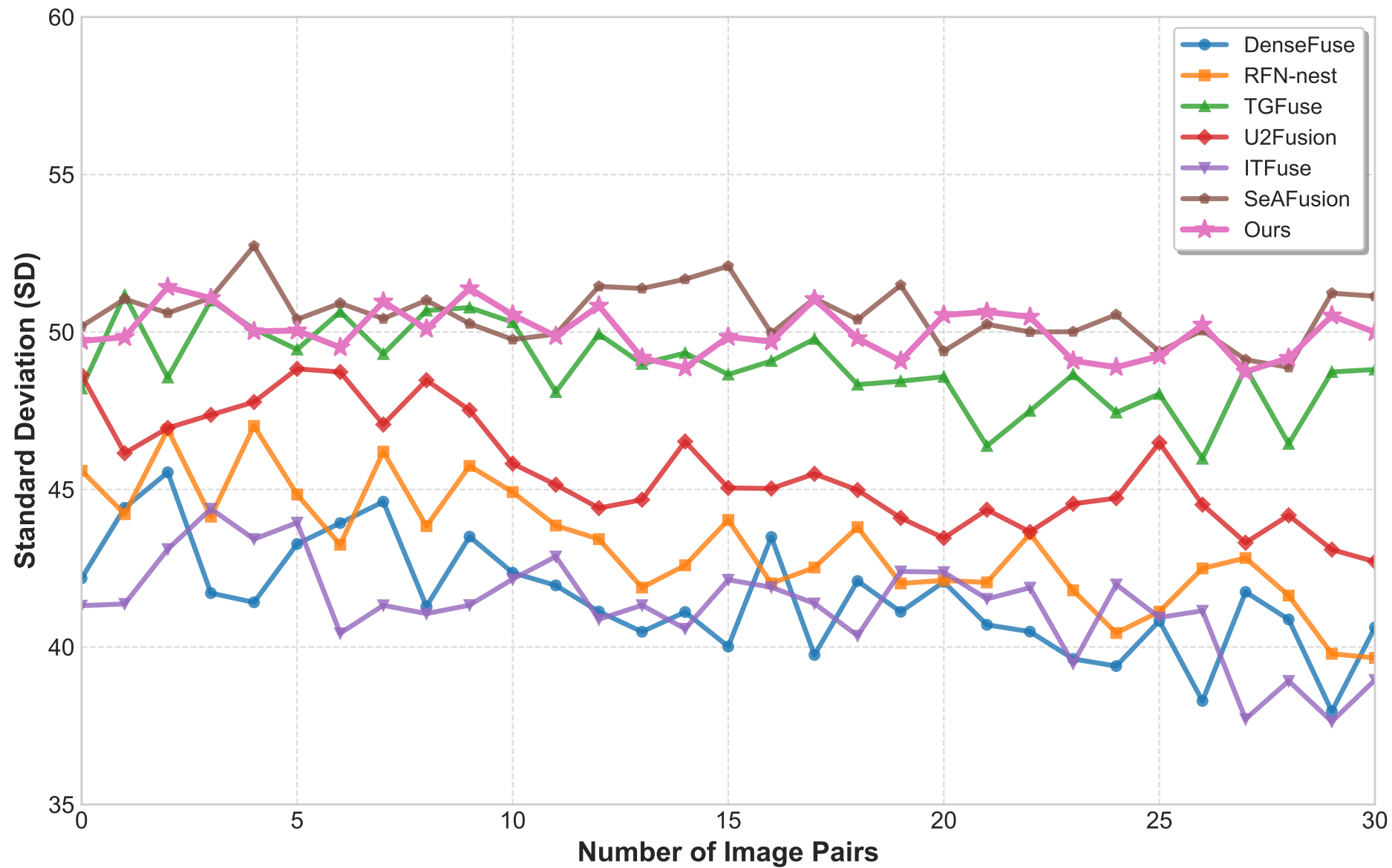
Standard Deviation (SD) Comparison (Higher is Better)
