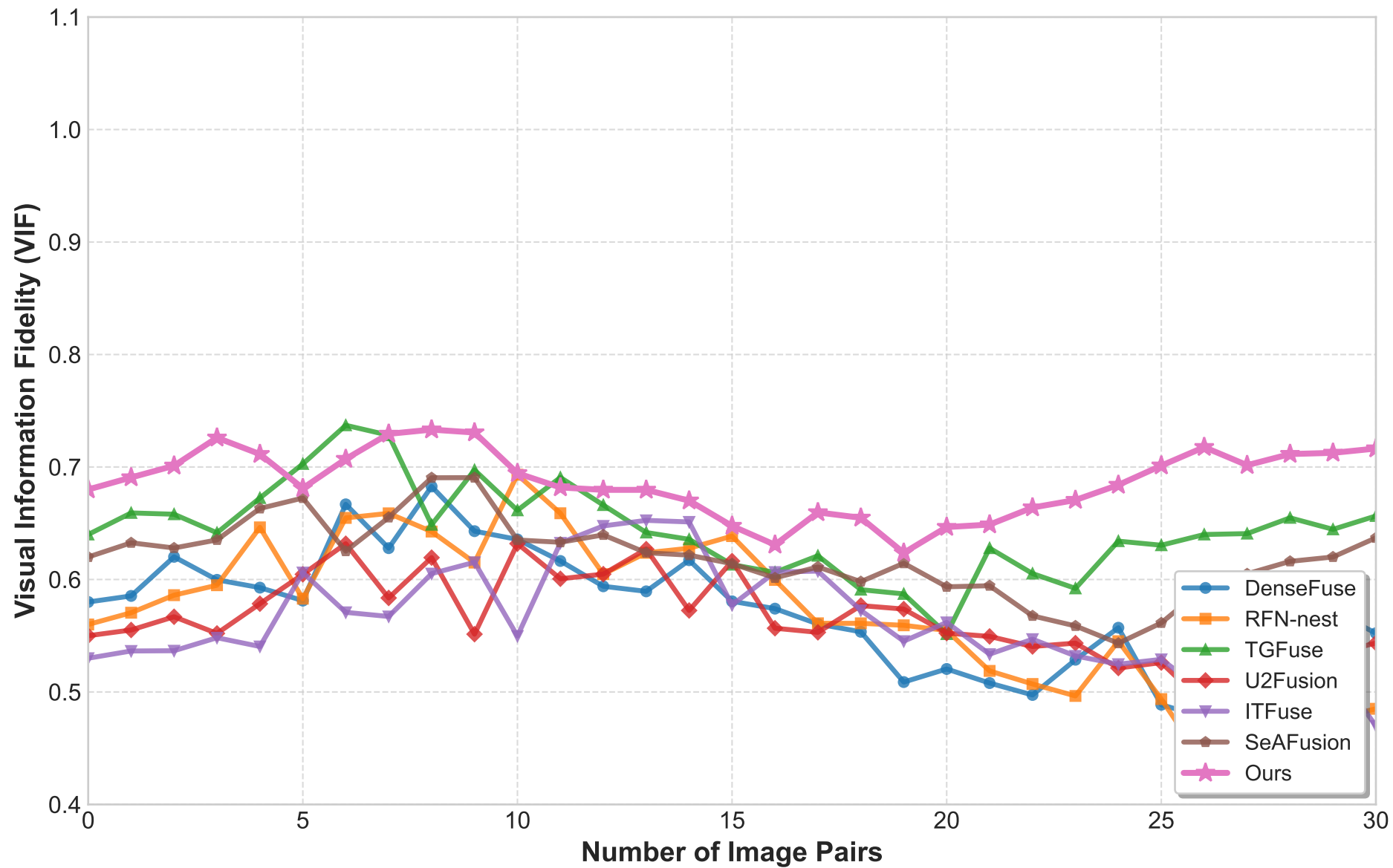
Visual Information Fidelity (VIF) Comparison (Higher is Better)
