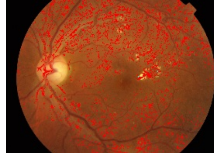
Grad-CAM attention
