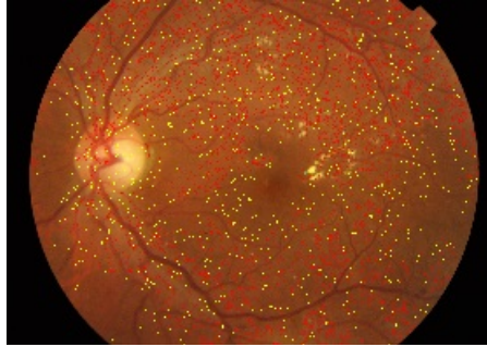
Annotated lesions
