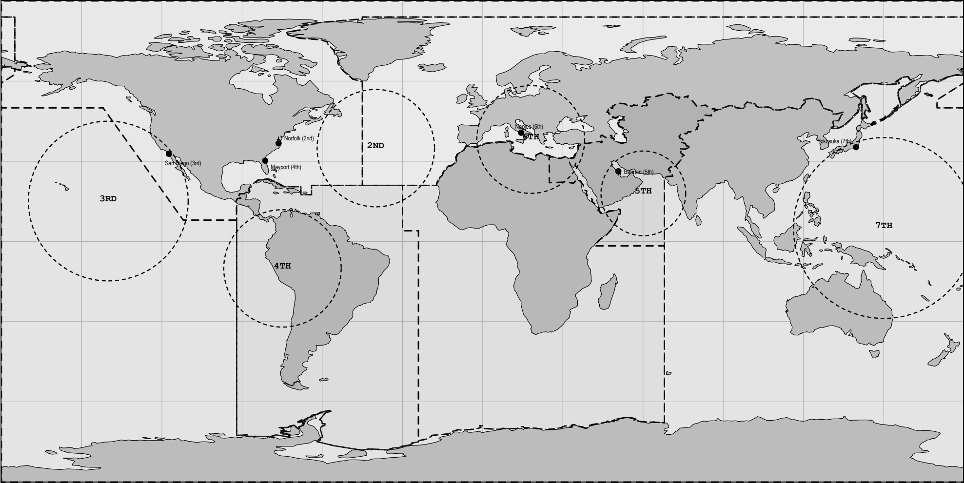
Coastlines: Natural Earth (public domain), equirectangular projection. Long dashes = combatant-command AOR boundaries (UCP, from source GeoJSON); short-dash ellipses = approximate fleet operating areas. • = fleet headquarters. 10th Fleet (cyber) has no geographic AOR.
