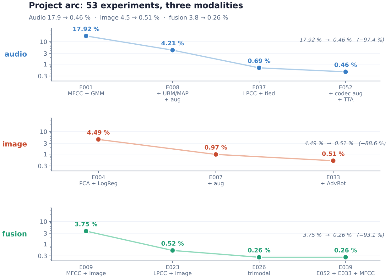
Figure 6: Project arc across 53 experiments. Each modality flagship dropped roughly two orders of magnitude from its anchor. Audio: 17.92 → 0.46 % (−97 %). Image: 4.49 → 0.51 % (−89 %). Fusion: 3.75 → 0.26 % (−93 %).
