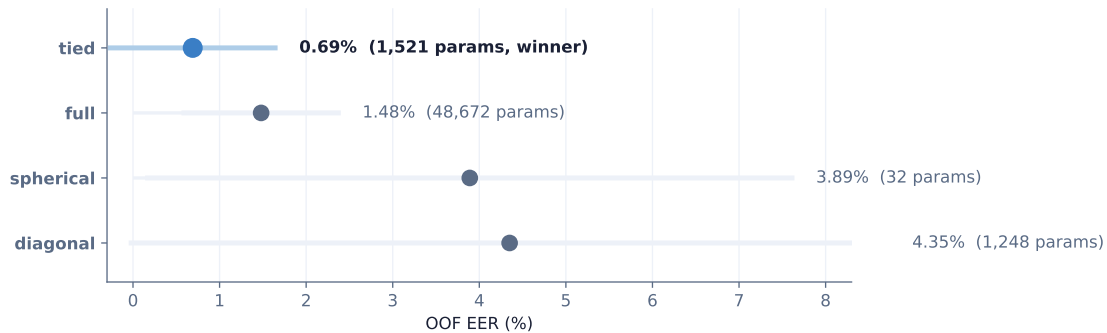
Figure 1: GMM covariance ablation: tied covariance is 6 \times better than diagonal at only ~20 % more parameters.
