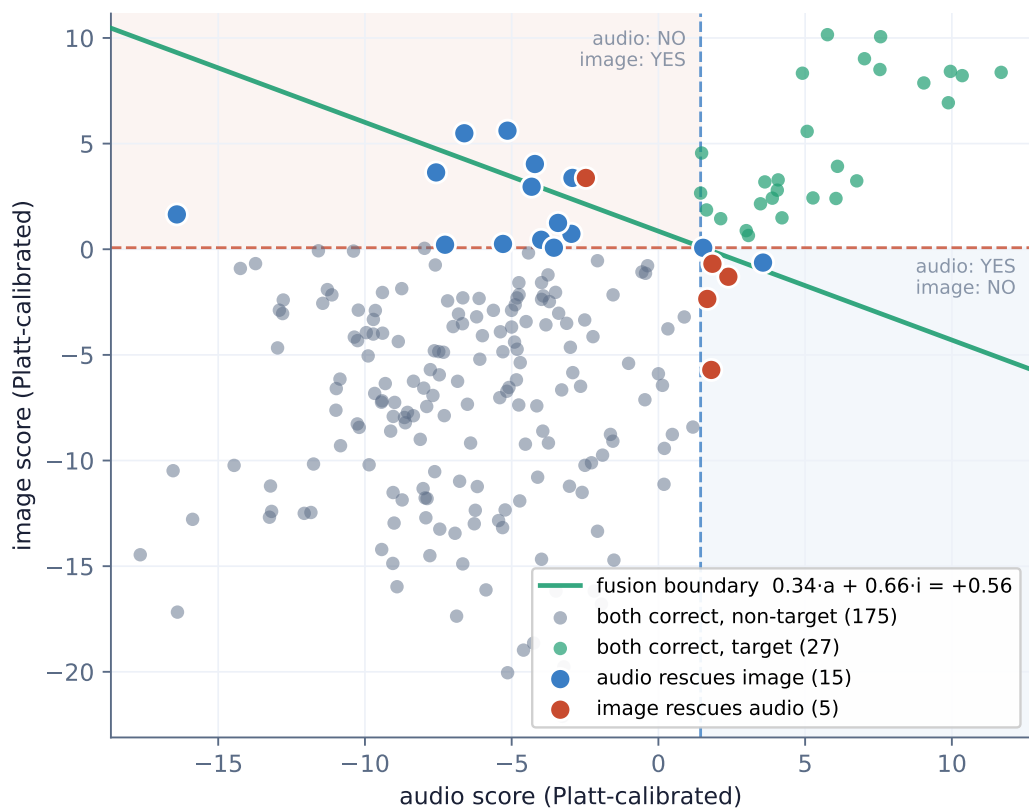
Figure 5: Audio \times image complementarity at per-stream EER thresholds: 15 samples are rescued by audio alone, 5 by image alone, none are missed by both. This disjoint failure pattern is exactly what makes weighted-sum fusion reach 0 errors.
