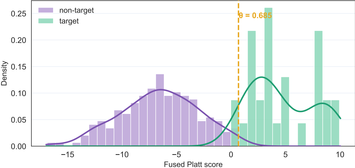
Fused OOF score distribution — E039 (222 trials)
