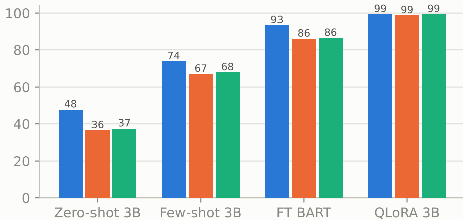
Exact match (%)
