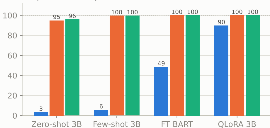
Sequence validity (%)
