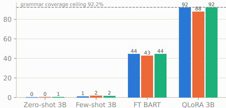
Exact match (%)
