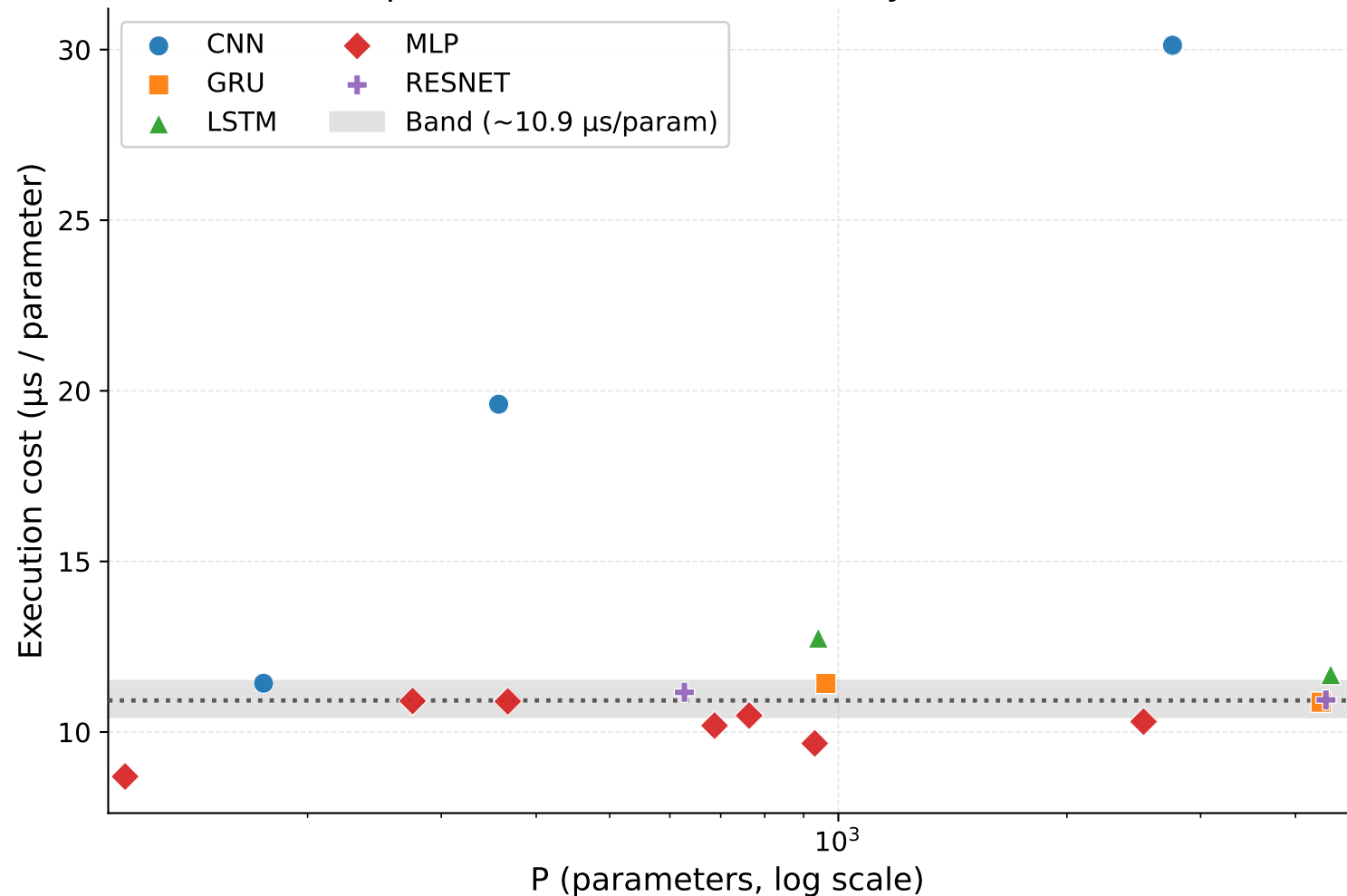
Per-parameter execution cost by architecture
