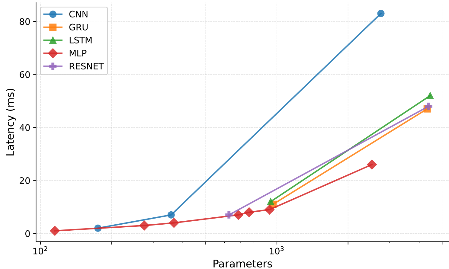
Inference Time vs Model Size
