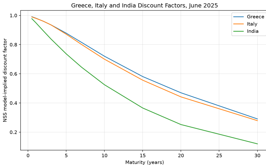
Figure 1: Automatically generated NSS model-implied Greece–Italy–India discount-factor comparison.
