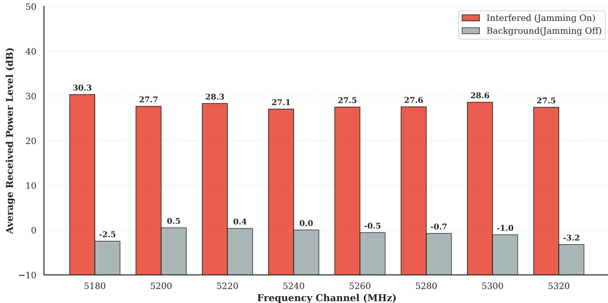
Comparison of Channel Power: Jammed vs. Background
