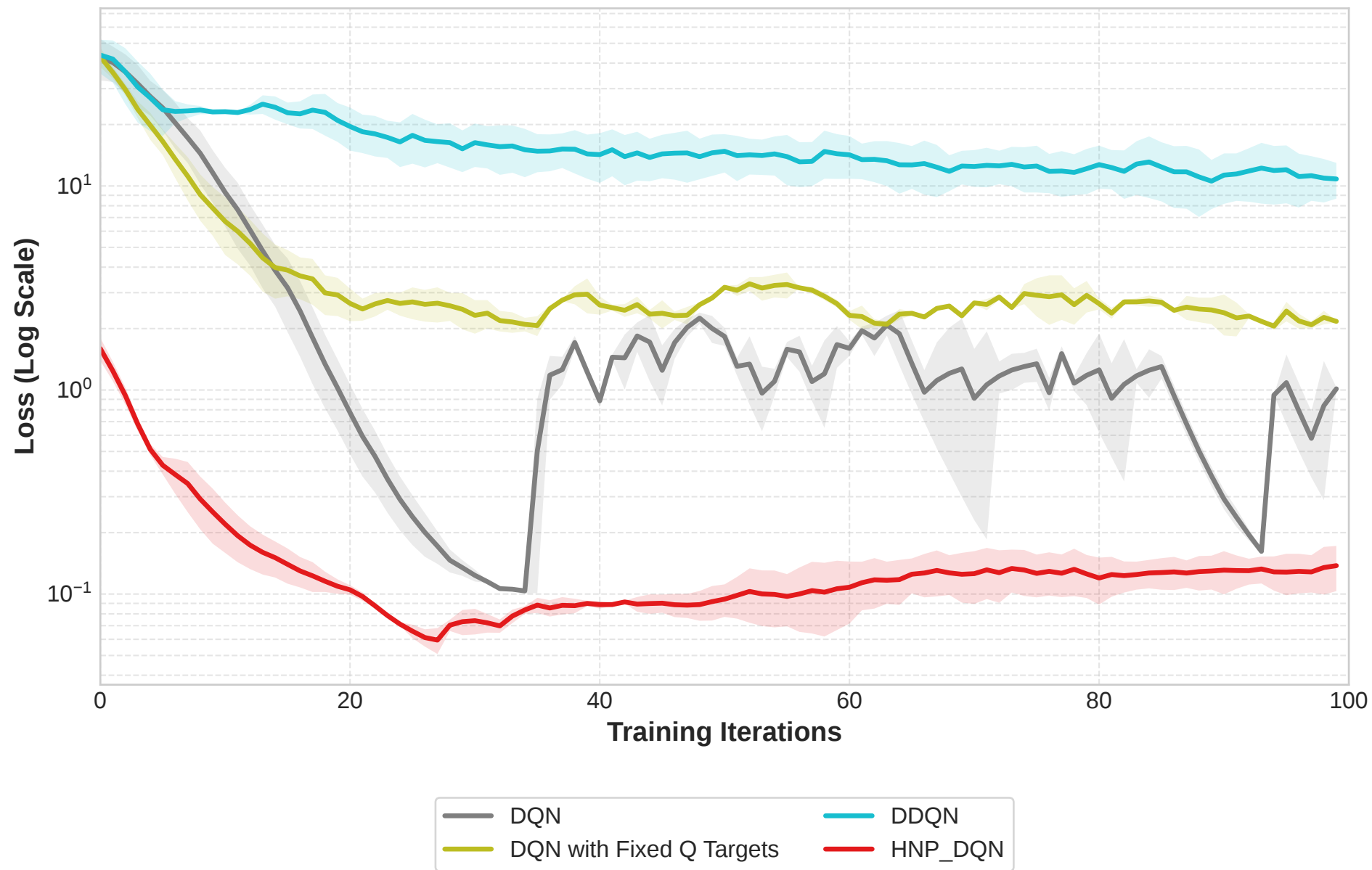
Initial Loss Dynamics (Random)
