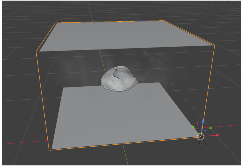
Figure 3.4: Planes added to the mesh in Blender to correspond to the bounding box of the volume.
