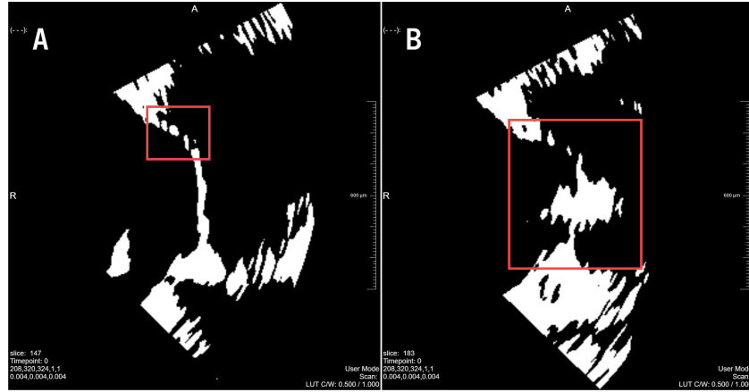
Figure 3.3: Thresholded ultrasound slices illustrating segmentation artifacts in the valvular material. (A) Discontinuity of the segmented membrane near the valve edge. (B) Substantial noise and false segmentation within the central region. Regions of interest are highlighted by red boxes.
