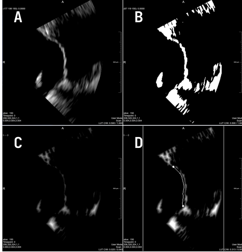
Figure 3.2: (A) Original ultrasound image. (B) Ultrasound image with a threshold set at >0.2 . (C) Ultrasound image after the Euclidean Distance Transform. (D) Mesh mapped onto the Euclidean Distance Transformed image — all images captured from an identical slice
