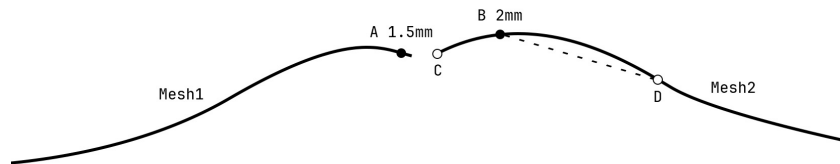
Figure 3.7: Schematic illustrating the use of Euclidean distance in IDW thickness interpolation. Although vertex C lies on Mesh2, it is closer to measurement A on Mesh1 than to measurement B on its own leaflet. Interpolating the leaflets separately prevents this influence across the gap. Within Mesh2, the dashed straight-line distance between B and D closely approximates the distance along the shallow surface curvature.
