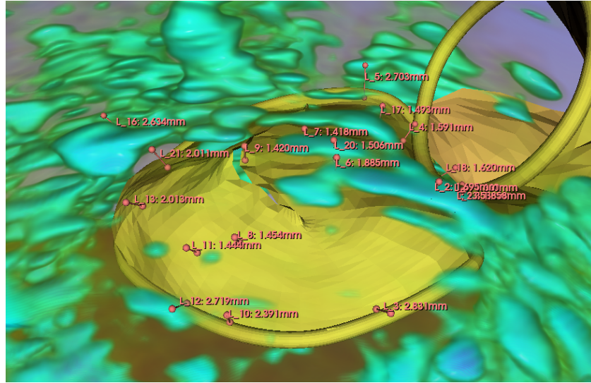
Figure 3.5: Valve mesh with volume and locations of the manual thickness measurements on the leaflets meshes from 3D-Slicer. Mesh depicted in yellow, ultrasound volume in blue/turquoise and measurement points in red
