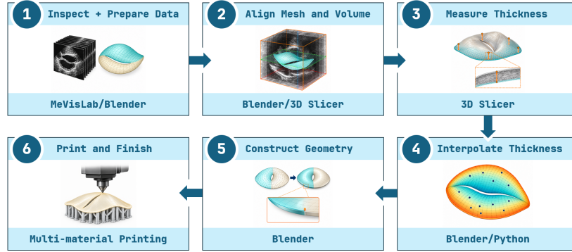
Figure 3.1: Mitral valve reconstruction and fabrication pipeline schematic. Illustrations generated using ChatGPT from methodological descriptions and refined through iterative prompting [Ope26].
