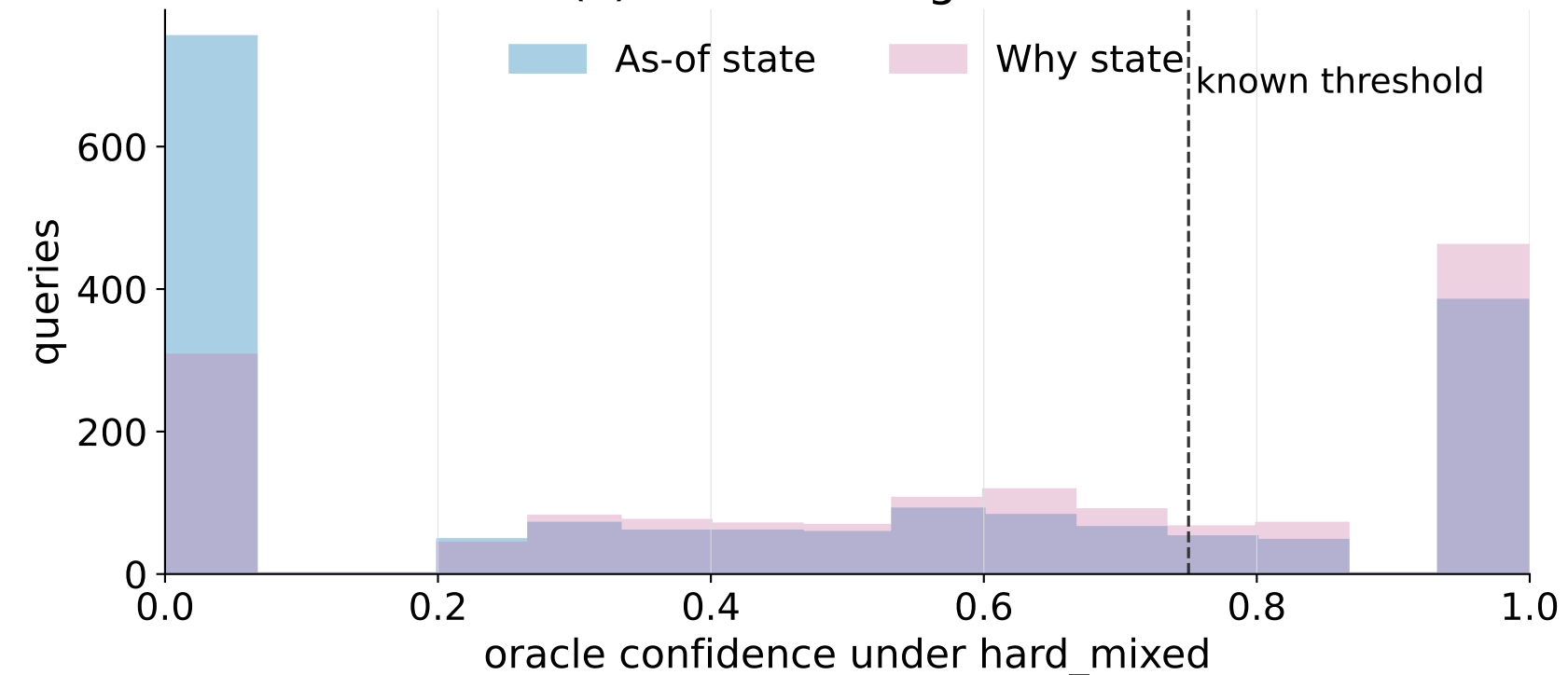
(c) Confidence gradient
