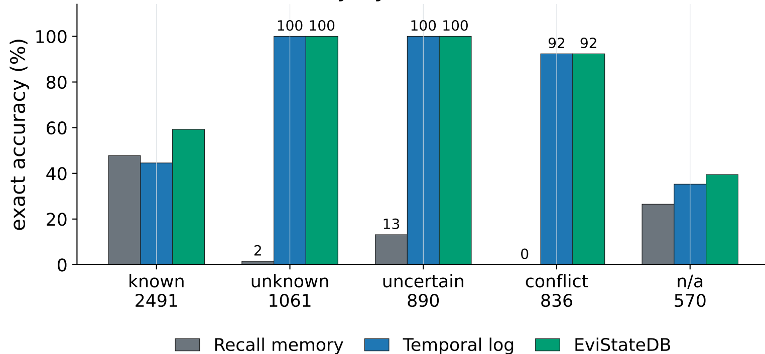
(a) Accuracy by oracle answer status
