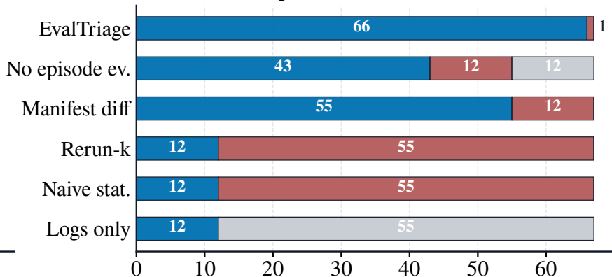
(b) Method comparison
