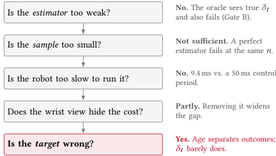
Figure 13: Independent controls eliminate estimator, sample-size, and compute explanations, leaving the scheduling target as the surviving diagnosis.
