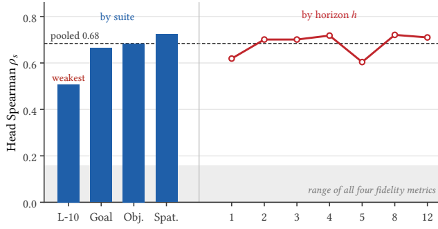
Figure 8: Decision relevance is predictable across suites and horizons; LIBERO-10 is weakest and has the highest operating-point cost.
