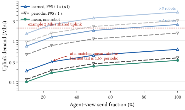
Figure 17: Event triggering is burstier, and encoded demand is sublinear in send fraction.
