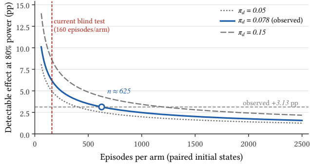
Figure 12: The blind test resolves roughly 6.2 pp; resolving the observed 3 pp gap would require about 625 episodes per arm.
