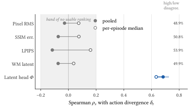
Figure 7: Fidelity metrics provide no stable ranking, whereas the latent head lies well outside their band.
