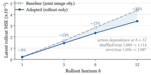
Figure 4: Dropping the image objective increasingly improves rollout error with horizon; one-step reconstruction selects the wrong predictor.
