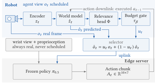
Figure 1: ActDelta schedules the agent view while wrist view and proprioception remain current in closed loop.
