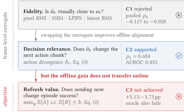
Figure 2: The three questions the paper separates. Fidelity does not rank decision relevance (C1); decision relevance is learnable offline (C2); neither buys refresh value in closed loop (C3).
