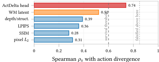
(b) which distance ranks decision impact
