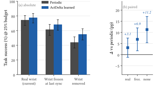
Figure 16: Removing wrist-view recovery widens the paired learned–periodic gap.
