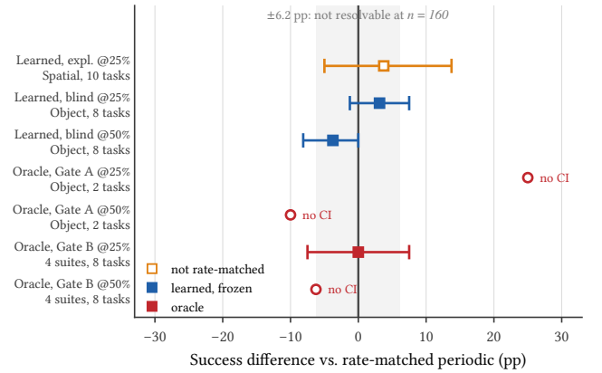
Figure 11: No rate-matched arm beats periodic sampling; the only large effect spends 3.95 additional send-rate points.
