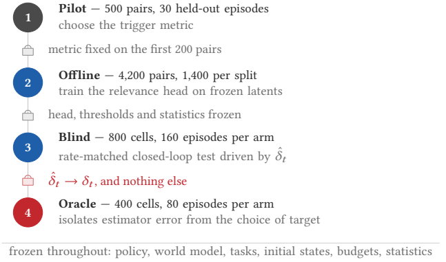
Figure 3: Four frozen stages isolate metric choice, relevance learning, blind testing, and the oracle target.
