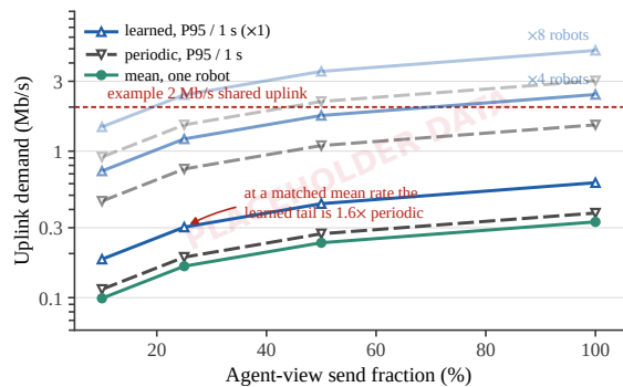
Figure 17: [PLACEHOLDER DATA] Send fraction is not bandwidth. Event triggering produces a burstier uplink than periodic sampling at the same mean rate, and demand scales sublinearly with send fraction because sparse sampling reduces inter-frame prediction gain. The shared-capacity line binds only once several robots share the link.
