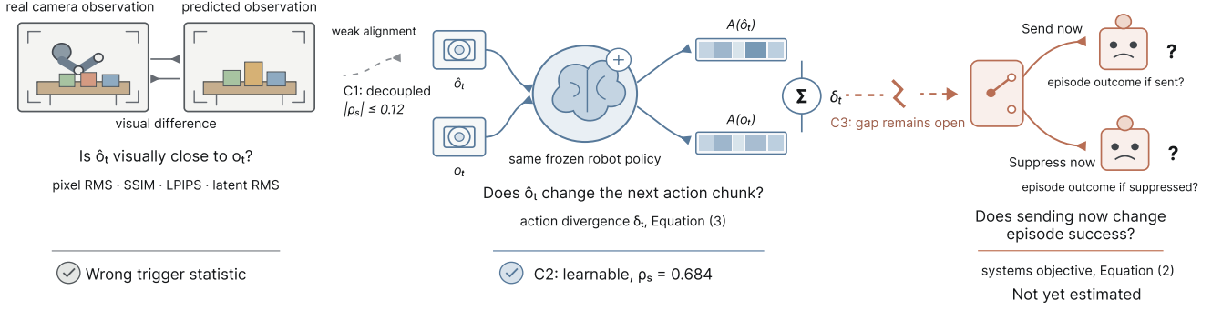
Figure 2: Three objectives separate reconstruction fidelity, decision relevance, and episode-level refresh value.
