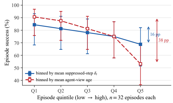
Figure 15: Observation age separates outcomes more sharply than action divergence ( n = 32 episodes per bin).
