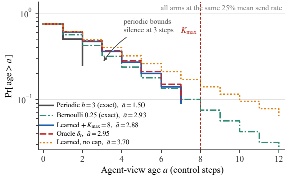
Figure 14: At an identical mean send rate, threshold triggering concentrates transmissions and leaves a heavier observation-age tail than periodic sampling—and, from an age of one step through six, than an unbiased coin at the same rate, which is the comparison that carries the argument. The maximum-silence safeguard truncates but does not remove the excess. Periodic and Bernoulli curves are exact, not measured, and bracket the range any scheduler at this rate can occupy.
