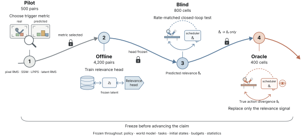
Figure 3: The frozen evaluation advances from pilot metric selection and offline head training to rate-matched blind and oracle tests.
