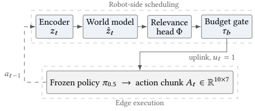
Figure 1: ActDelta refreshes the agent view when predicted policy relevance exceeds a budgeted threshold. The wrist view and proprioception are always current; only the agent view is suppressible. The dashed return path is the closed loop: the executed action a_{t-1} conditions the next rollout, which is why a scheduler cannot be evaluated on per-frame ranking alone.
