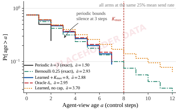
Figure 14: [PLACEHOLDER DATA] At an identical mean send rate, threshold triggering concentrates transmissions and leaves a heavier observation-age tail than periodic sampling—and, from an age of one step through six, than an unbiased coin at the same rate, which is the comparison that carries the argument. The maximum-silence safeguard truncates but does not remove the excess. Periodic and Bernoulli curves are exact, not measured, and bracket the range any scheduler at this rate can occupy.
