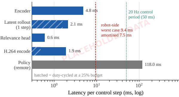
Figure 18: [PLACEHOLDER DATA] The robot-side trigger path costs a small fraction of one remote policy call and fits comfortably inside the control period, so the scheduling question is not limited by local compute.
