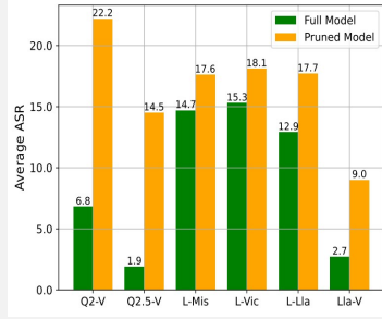
Fig. 1: The Average ASR (lower values indicate higher safety) of full baselines versus pruned models
