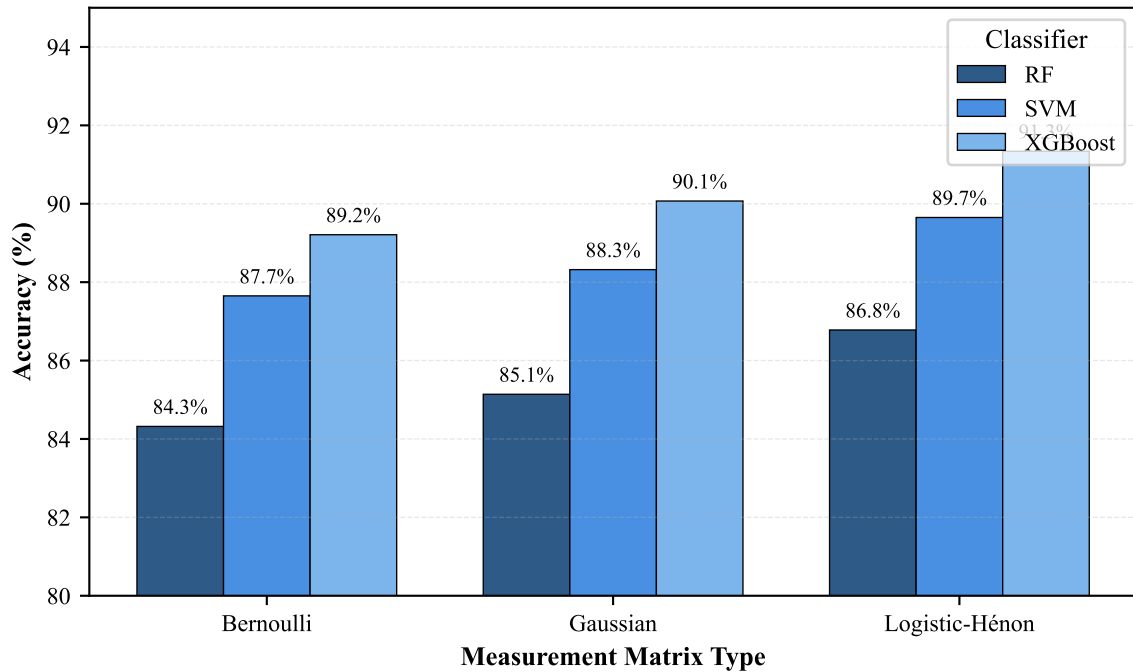
Accuracy Comparison at 25% Compression Ratio
