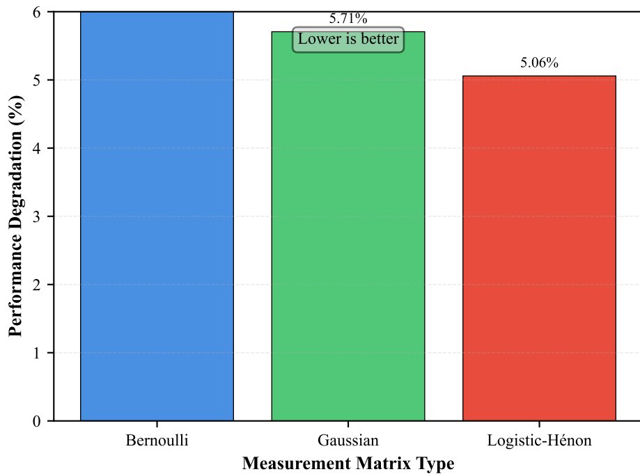
Accuracy Loss from 25% to 75% Compression
