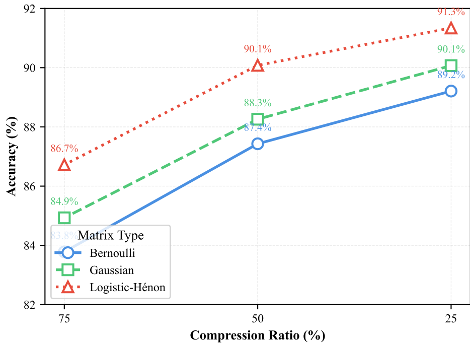
Accuracy vs Compression Ratio (XGBoost Classifier)
