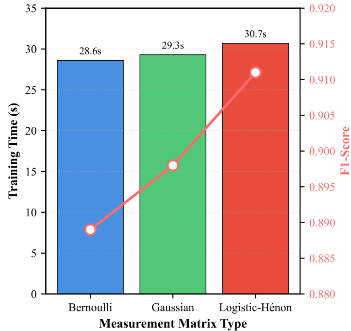
XGBoost Training Time at 25% CR
