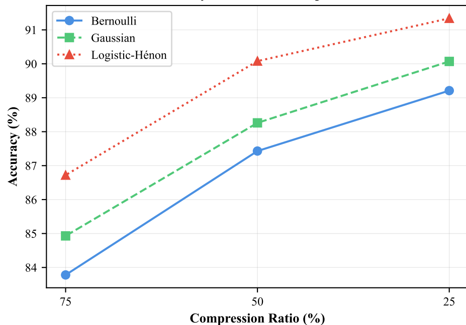
Accuracy Trend with Compression
