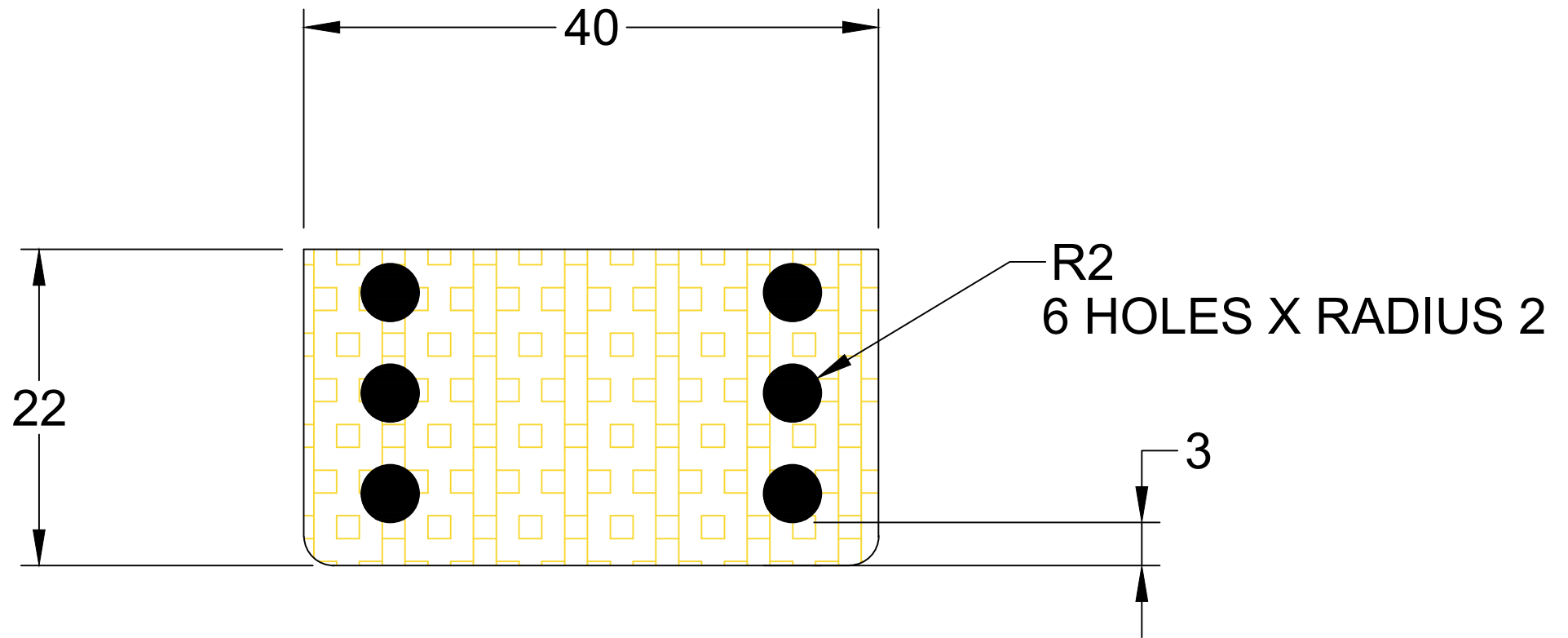
TOP VIEW OF CLAMP
