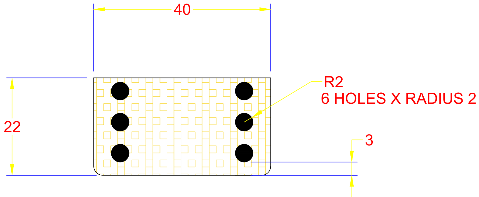
TOP VIEW OF CLAMP
