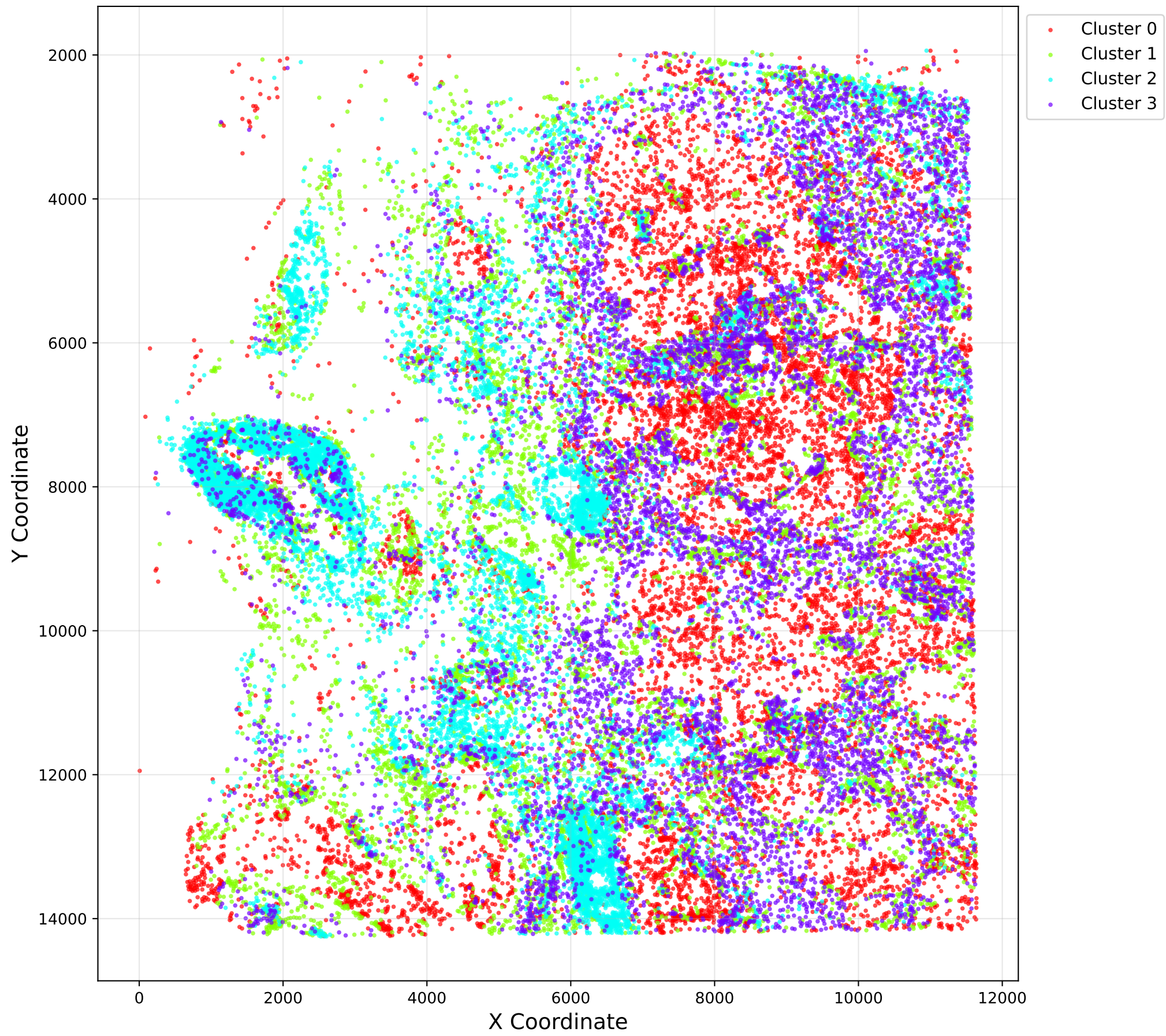
LDA Spatial Clustering (K=4, 37817 cells)
