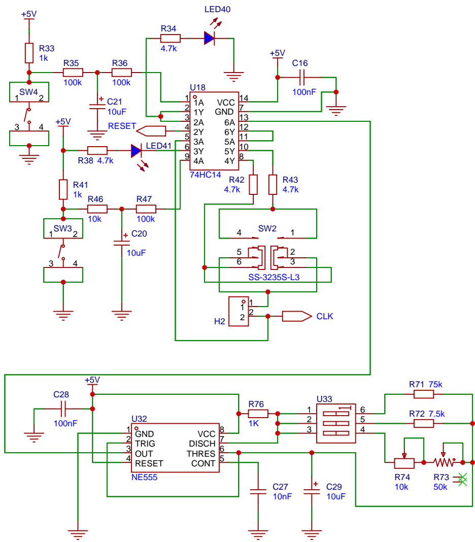
CLOCK&RESET
