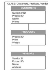
Object-oriented Data modeling technique
