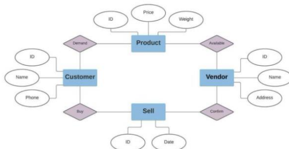
Entity-relationship Data modeling technique
