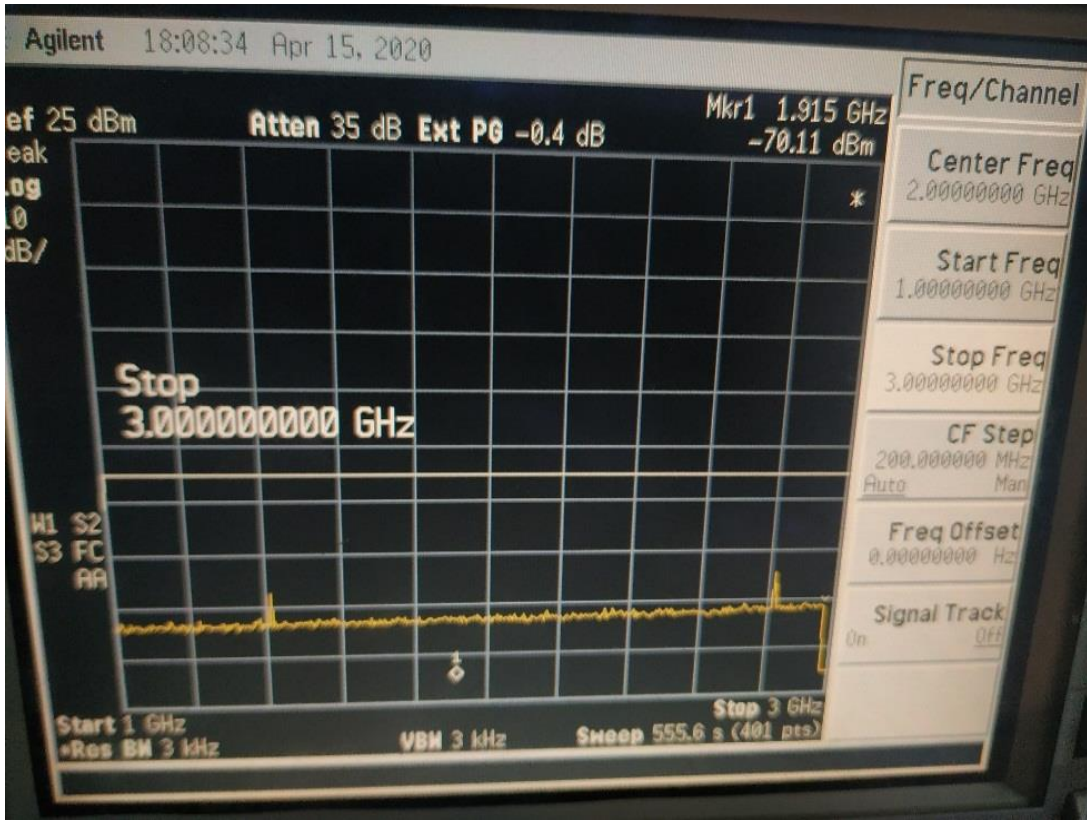
Figure 8 Harmonic(1GHz~3GHz)@Frf=470MHz, TXOP=22dBm
