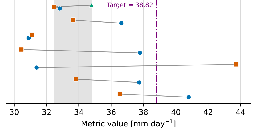
Spatial SD of annual precipitation (closer to HR is better)
