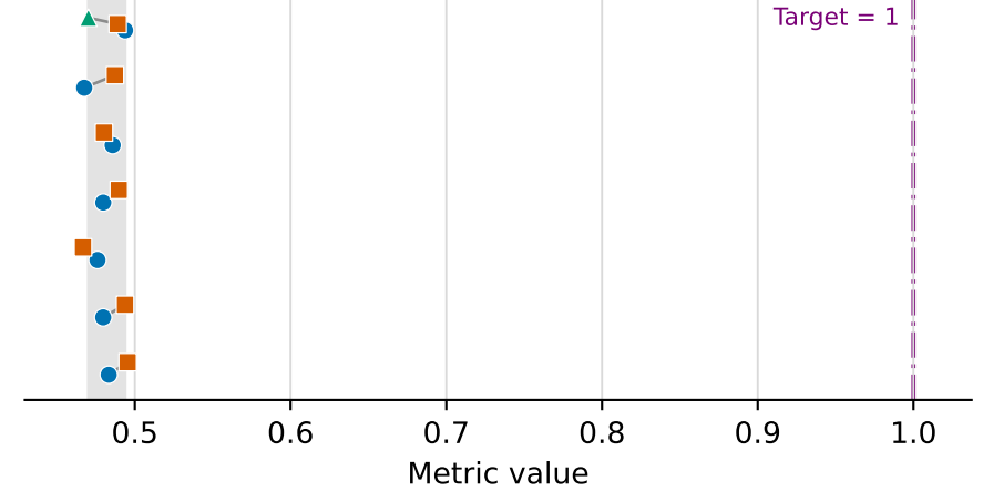
99.9th percentile (closer to HR is better)
