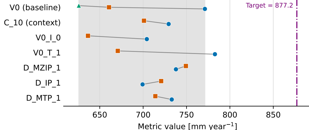
Mean annual precipitation (closer to HR is better)
