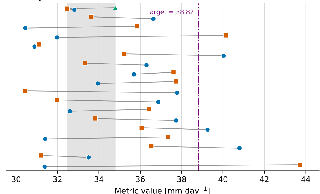
99.9th percentile (closer to HR is better)
