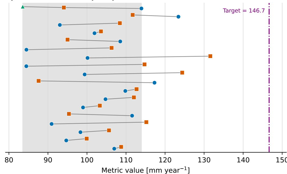
Spatial SD of annual precipitation (closer to HR is better)
