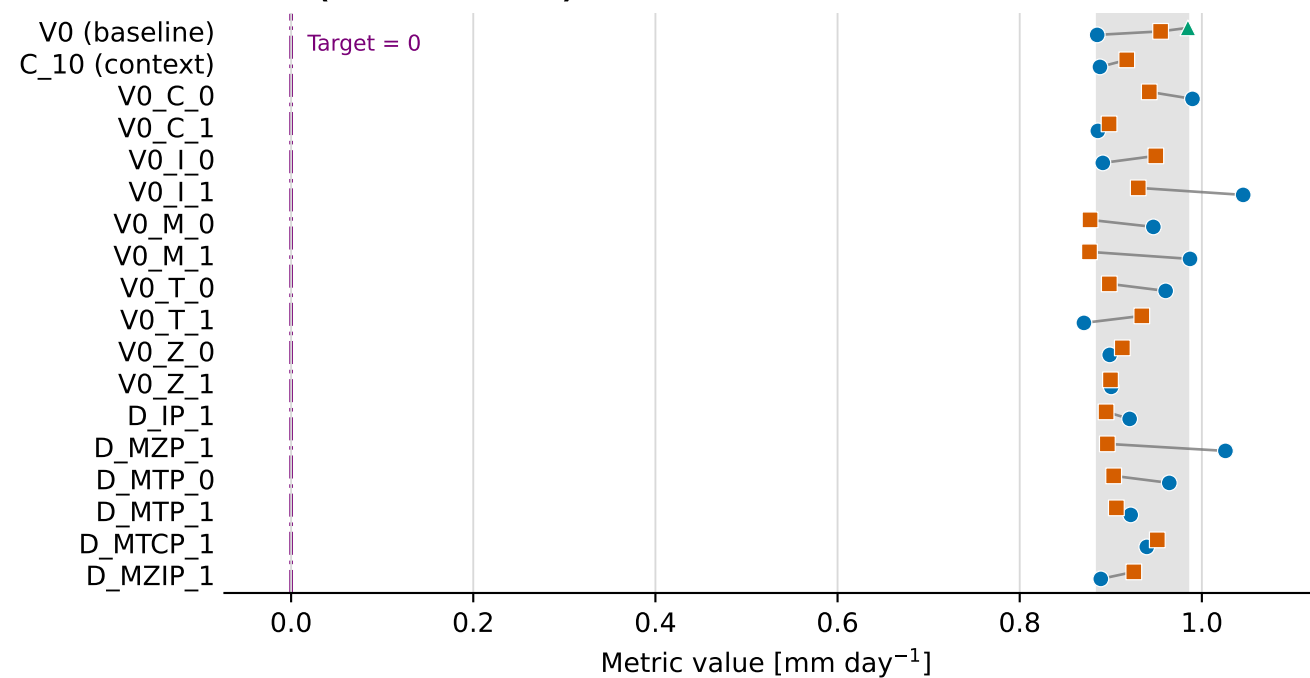
CRPS (lower is better)
