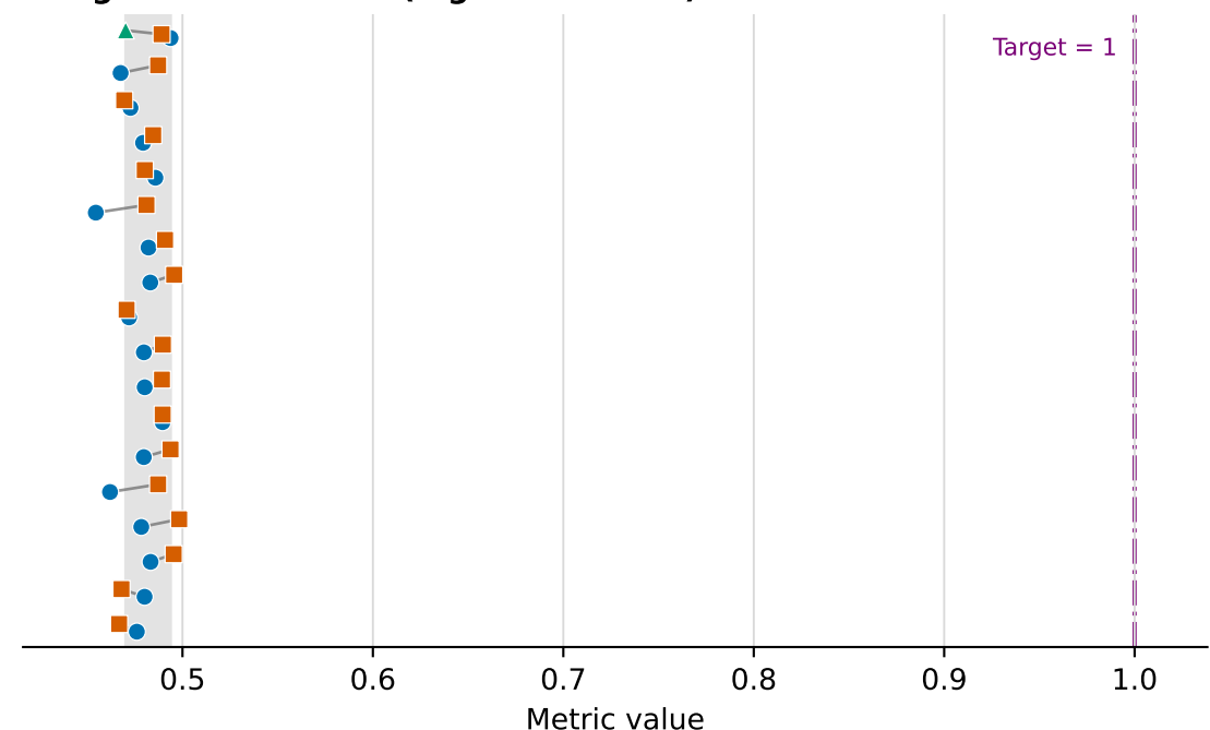
Integrated skill score (higher is better)
