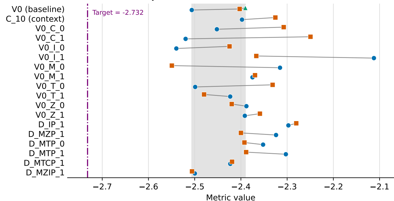
Mid-scale PSD slope (closer to HR is better)
