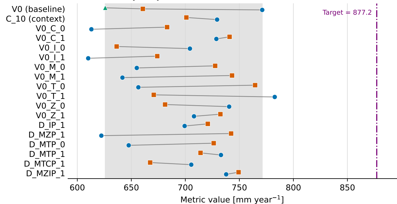
Mean annual precipitation (closer to HR is better)
