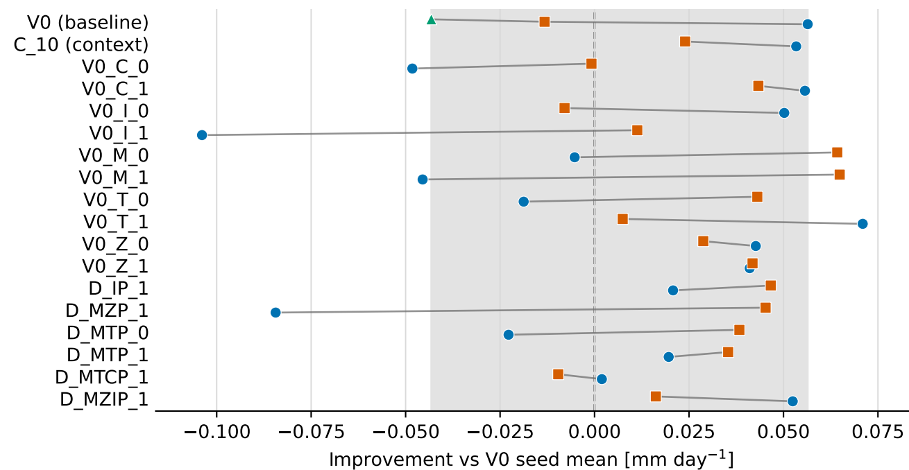
CRPS
