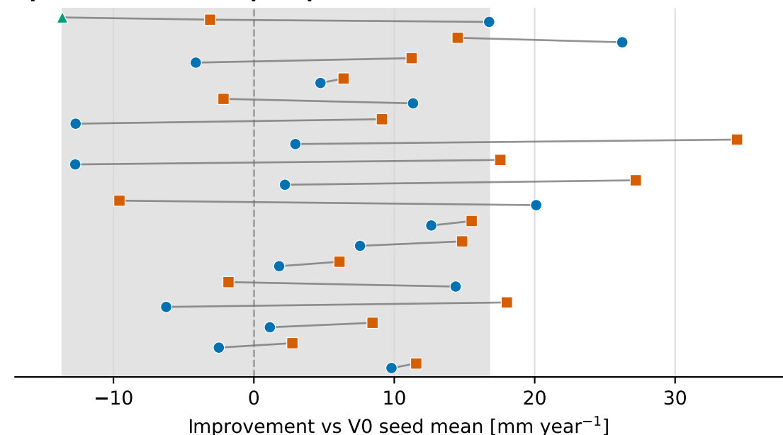
Spatial SD of annual precipitation
