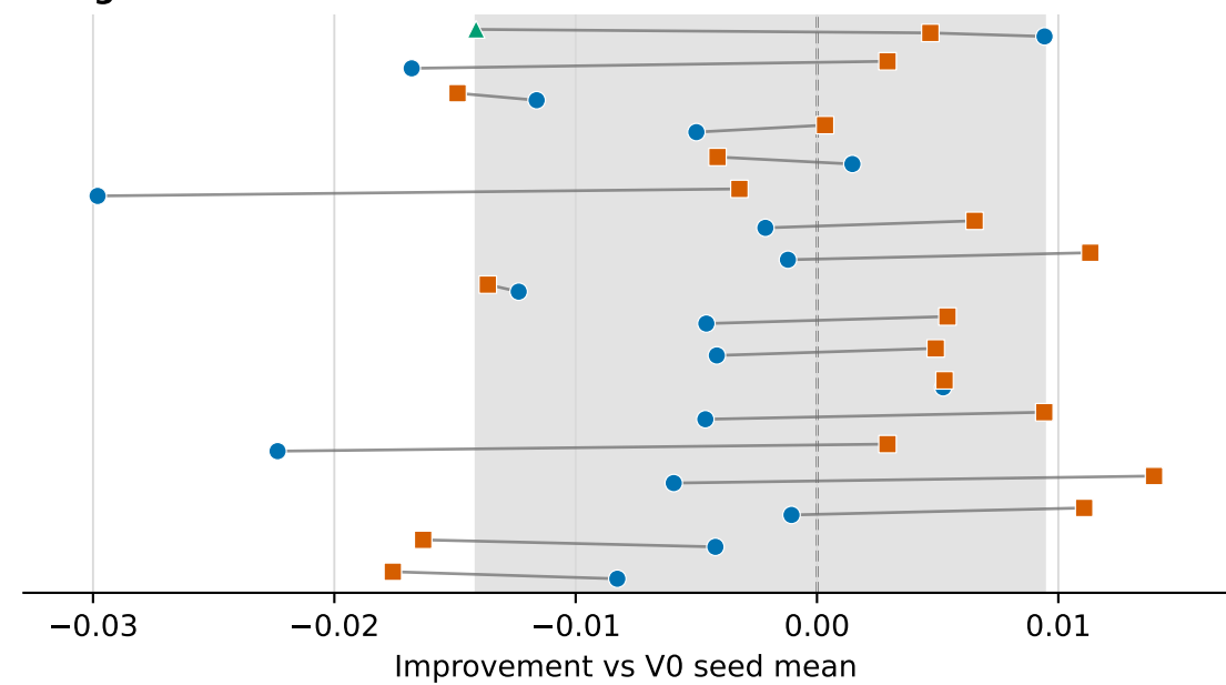
Integrated skill score
