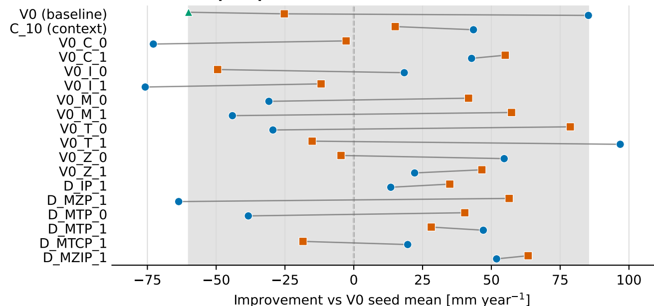
Mean annual precipitation
