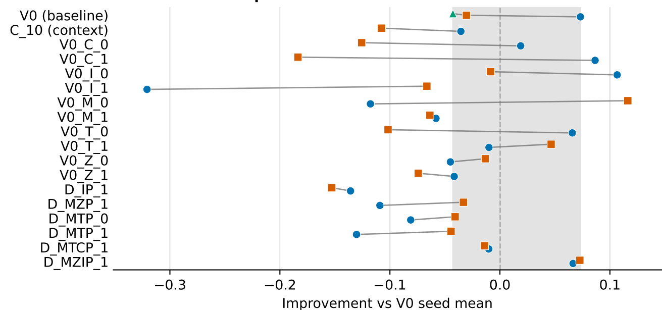
Mid-scale PSD slope
