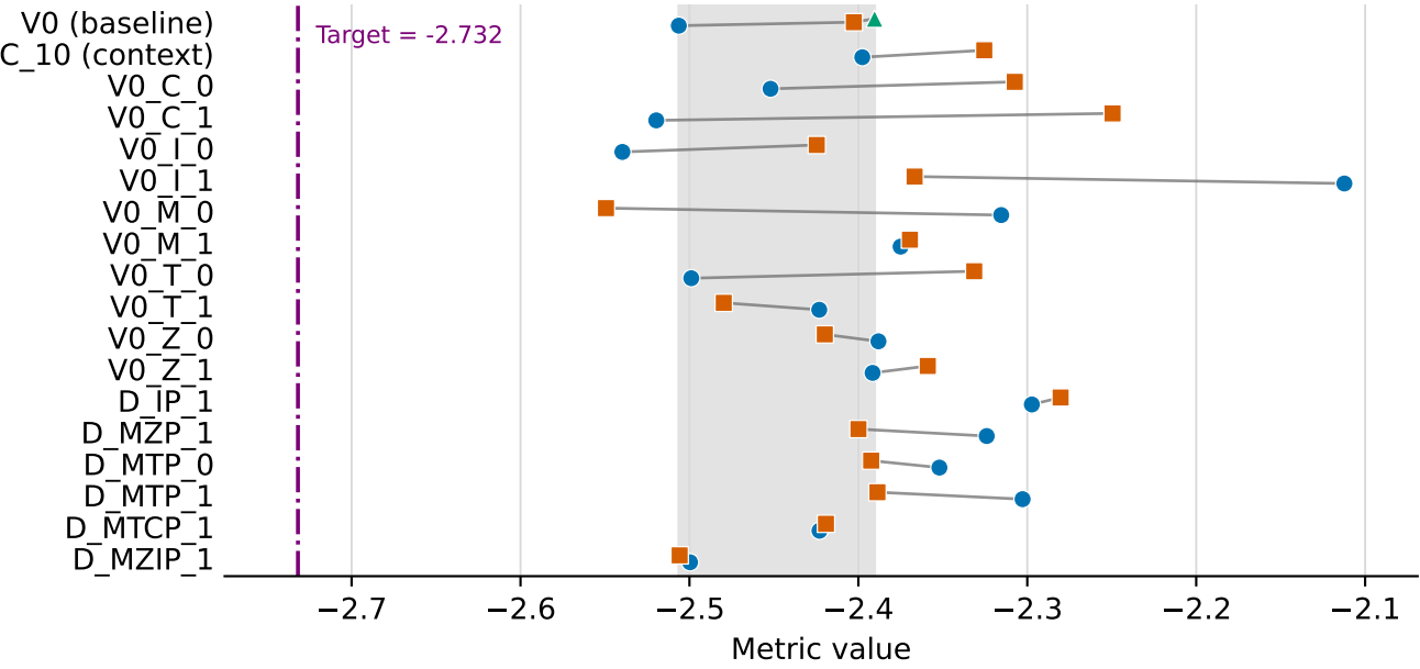
Mid-scale PSD slope (closer to HR is better)
