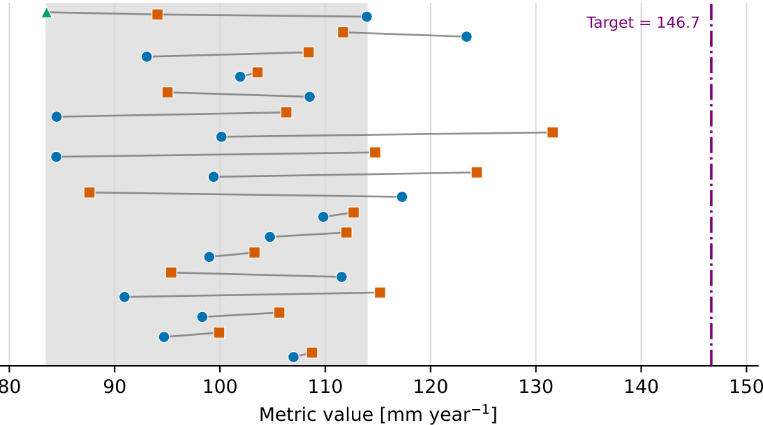
Spatial SD of annual precipitation (closer to HR is better)
