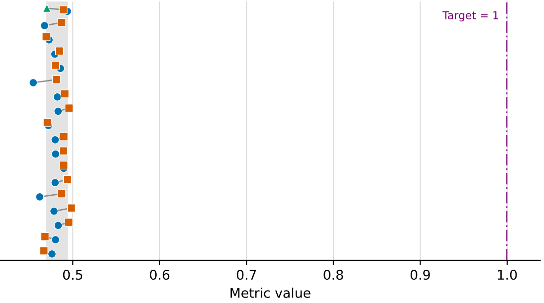
Integrated skill score (higher is better)
