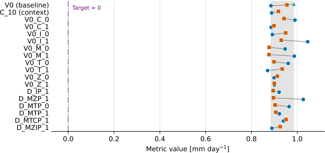
CRPS (lower is better)
