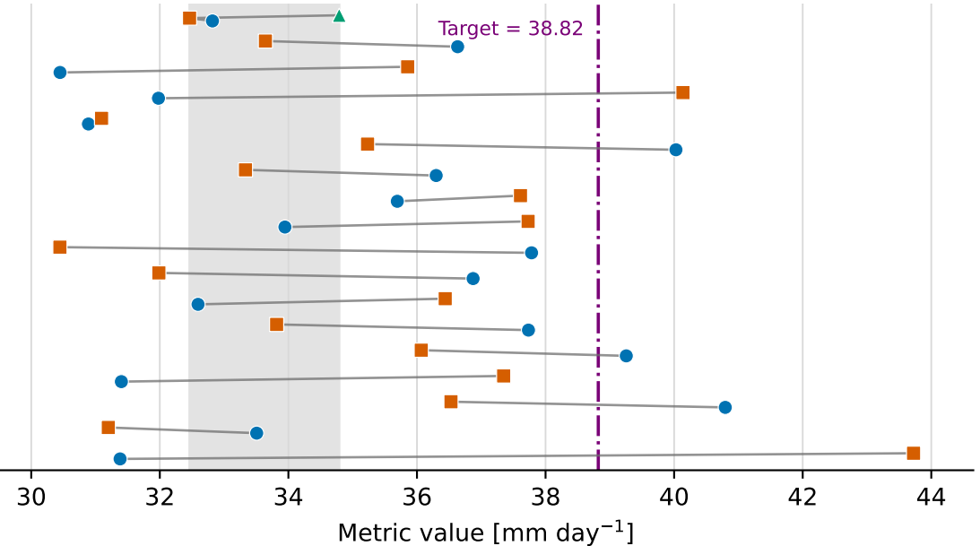
99.9th percentile (closer to HR is better)
