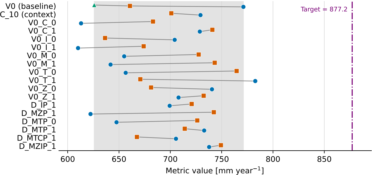
Mean annual precipitation (closer to HR is better)
